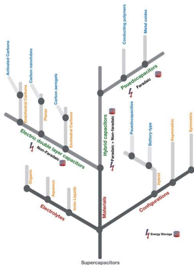
Fig. 2 An overview of the taxonomical classification of supercapacitors. The lightning bolt symbol represents energy and the cylindrical stack represents the storage.
