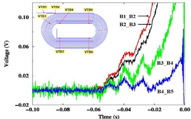
Fig. 5. Voltage growth in some segments of coil 13 OL. The inset shows the location of the voltage taps. Each segment is identified by its voltage tap pair. The voltage of segments B1_B2, B3_B4, and B4_B5 have been scaled respectively 5, 10, and 10 times. Note the three “bumps” occurring at the same time in all segments.
