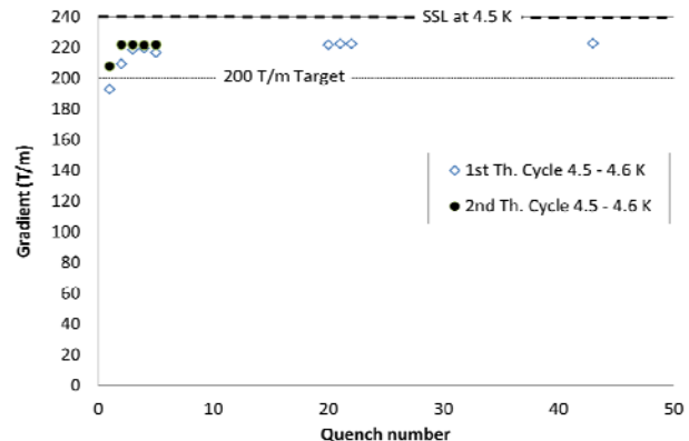
Fig. 1. Quench history of LQS01b 1 st and 2 nd thermal cycles. Only the quenches at 20 A/s ramp rate are presented.
