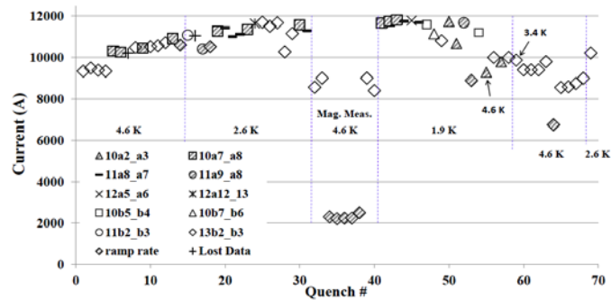
Fig. 3. Quench history of LQS02 showing the location of each quench start.
