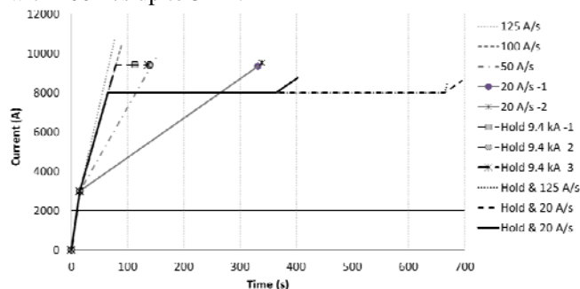
Fig. 7. Current vs. time in standard ramps to quench at constant rate, and in current holding tests. The quench occurred at the end of each line or where there is a marker (in case of tests repeated in the same conditions). All these tests were performed at 4.6 K.
