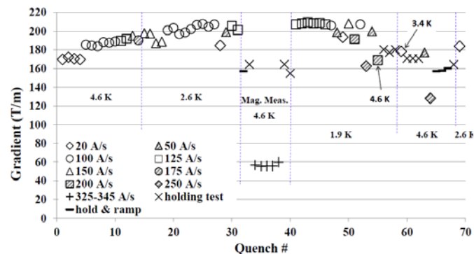
Fig. 2. Quench history of LQS02 showing bath temperature and current ramp rate.
