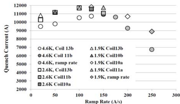
Fig. 4. Limiting coil (a = IL, b = OL) at different ramp rate and temperature.
