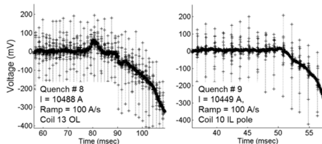
Fig. 6. VSDS signal at the start of a typical quench in coil 13 (left), and at the start of a typical training quench (right). Temperature was 4.6 K in both cases. In the plots there is a noise from the power supply with 720 Hz frequency. The actual signal is given by the thick lines.
