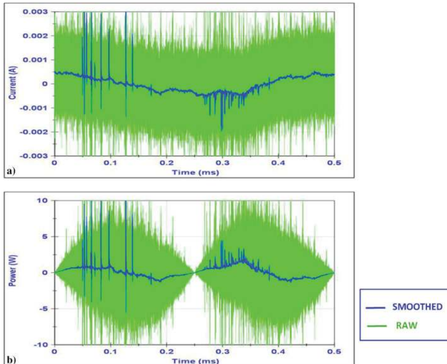
Fig. 15 Visual noise reduction with smoothing: a) current, and b) instantaneous power.
