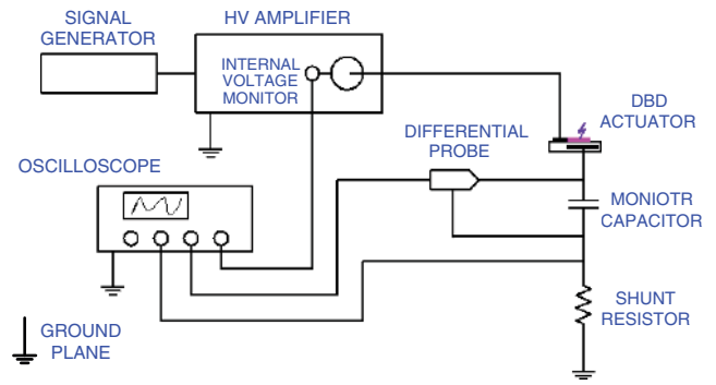
Fig. 6 Schematic of the test setup.
