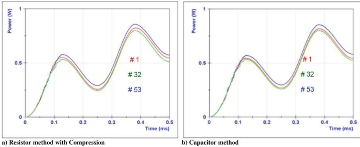
Fig. 20 Power evolution for three selected cycles out of 64 consecutive cycles (red: cycle 1; green: cycle 32; blue: cycle 53): a) shunt resistor method with compression, and b) monitor capacitor method.
