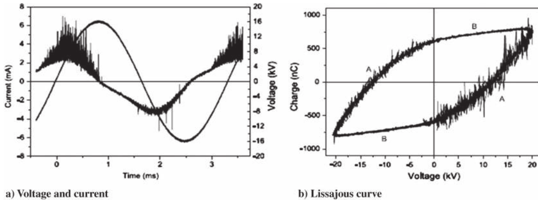
Fig. 3 Representations of a) applied voltage and current, and b) Lissajous curve (from Pons et al. [16], reprinted with permission).
