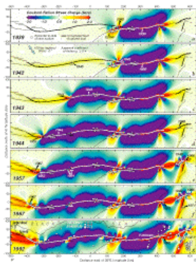
Fig. 4. Cumulative stress changes caused by large earthquakes and steady deep slip on the North Anatolian fault since 1939. In each panel, the epicenter of the next earthquake to rupture is circled. All but the 1943 epicenter lie in regions where the stress rose significantly, typically by 2-5 bars, owing to the foregoing shocks and deep fault slip. Relocated ISC earthquakes (Engdahl, et al., 1996) are shown in g, with the 1992 Erzincan aftershock sequence removed. Calculations are made in an elastic halfspace with a shear modulus of 3.15 \times 10^{11} dyne-cm -2 and Poisson's ratio of 0.25. Earthquake slip is assigned as in Fig. 1b, assumed to be uniform over 0-12.5-km depth. The fault was digitized and stress was sampled at 5-km increments, and is projected as in Fig. 1c so that the regional stress maintains nearly a fixed angle to the fault.
