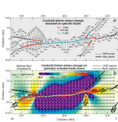
Fig. 3. Stress changes associated with the 1939 earthquake. (a) Coulomb stress change on major faults caused by the 1939 earthquake. Stress is resolved on the fault surface, projected in UTM coordinates, at a depth of 8 km. Faults are assumed to be vertical, except for the west end of the 1939 rupture, which dips 50° N. No information about the regional stress is needed for this calculation. The mean stress change along the future 1942 rupture is +1.4 bars. (b) Color gradients show the Coulomb stress change on optimally oriented vertical strike-slip faults at a depth of 8 km. The calculation assumes that the regional stress is 100 bars compression oriented 55° clockwise from the local Anatolian fault strike. Large rotations of the optimal planes are restricted close to the fault rupture, where the earthquake stress change is significant relative to the regional stress. Far from the 1939 rupture, rotation of the optimal planes is negligible.
