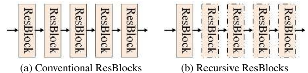
Figure 3. Implementations of f_{res} : (a) conventional ResBlocks and (b) recursive ResBlocks where one ResBlock is recursively unfolded five times.
