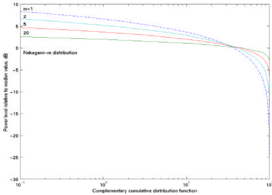
Fig. 2. Complementary cumulative distribution function of relative power level for Nakagami m-distribution.
