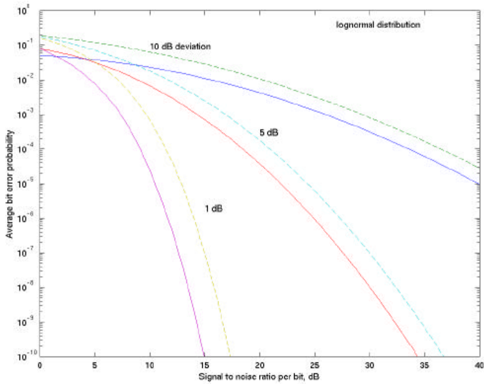
Fig. 4. Average bit error probability of lognormal distribution channel for uncoded transmission as a function of the mean signal to noise ratio per bit; solid lines used for BPSK modulation and dashed lines for DQPSK modulation.
