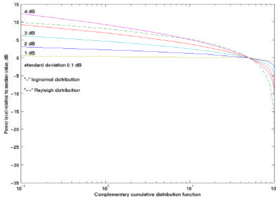
Fig. 1. Complementary cumulative distribution function of relative power level for lognormal distribution. Similar result for Rayleigh distribution is included.
