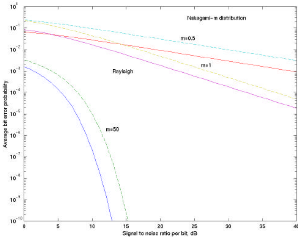
Fig. 3. Average bit error probability of Nakagami m-distribution channel for uncoded transmission as a function of the mean signal to noise ratio per bit; solid lines used for BPSK modulation and dashed lines for DQPSK modulation.
