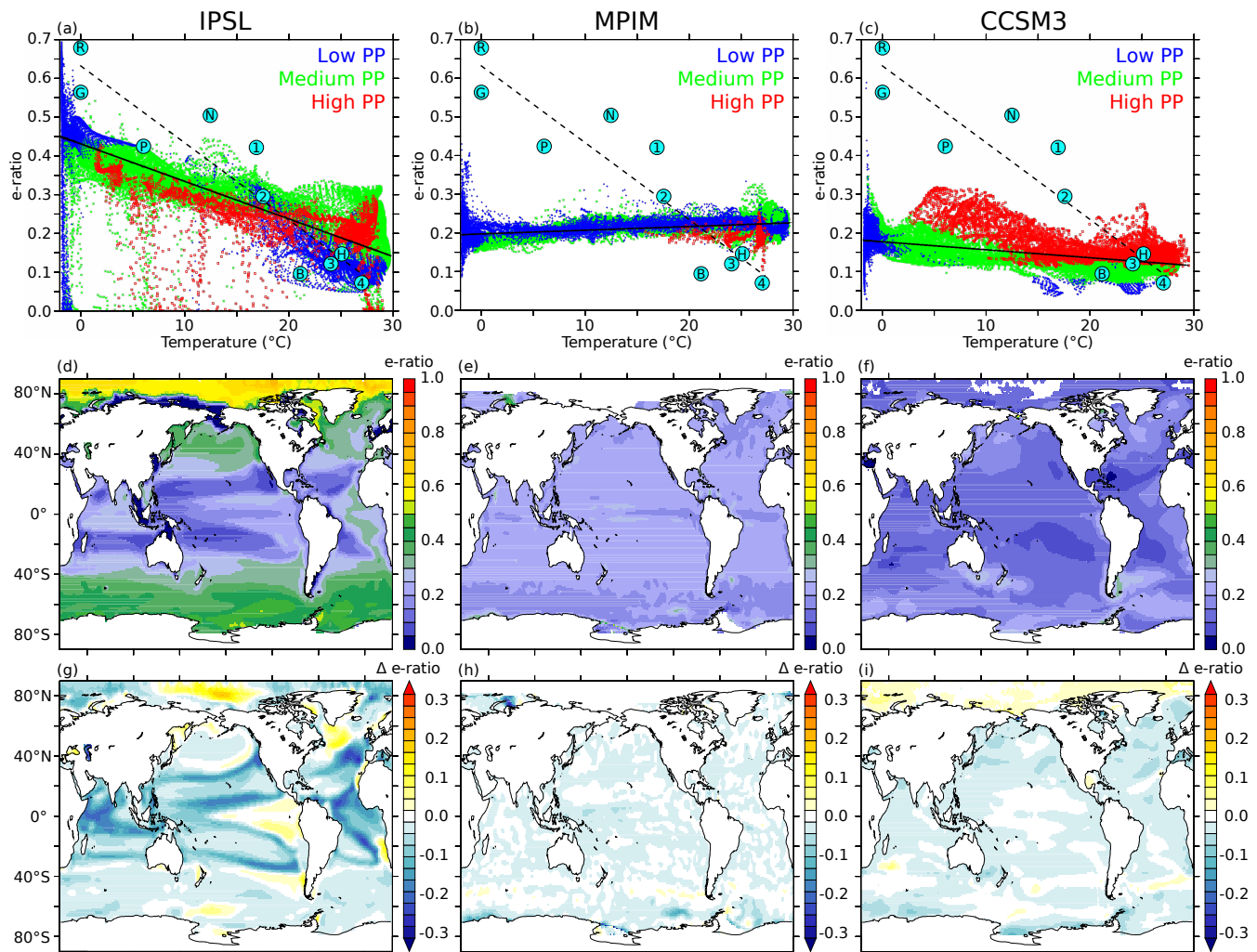
Fig. 3. Export ratio (e-ratio; EP:PP) simulated by the IPSL (left), MPIM (middle), and CCSM3 (right) models. The preindustrial (decadal mean 1860–1869) e-ratio is shown as a function of sea surface temperature ( a , b , c ). Each point represents one grid cell and the colors indicate low (blue; 10–150 mg C/m 2 /day), medium (green; 150–450 mg C/m 2 /day), and high (red; >450 mg C/m 2 /day) PP. Circles show field data (cf. Laws et al., 2000, Fig. 4) for the following locations: BATS (B), HOT and Arabian Sea (H), NABE (N), Peru-normal (1), Peru-El Niño (2), EqPac-normal (3), EqPac-El Niño (4), Ross Sea (R), Station-P (P), and Greenland polynya (G). The straight solid lines indicate the linear regression for IPSL ( r^2 = 0.58 , slope = -0.0097 ), MPIM ( r^2 = 0.21 , slope = 0.0010 ), and CCSM3 ( r^2 = 0.28 , slope = -0.0021 ), while the dashed line indicates the regression of the field data selected by Laws et al. (2000) ( r^2 = 0.86 , slope = -0.0198 ). Maps show the simulated e-ratio under preindustrial conditions ( d , e , f ) and the projected changes by the end of the 21st century under SRES A2 ( g , h , i ). Where PP is below a minimum threshold of 10 mg C/m 2 /day the e-ratio is not shown. In the CSM1.4 model the e-ratio is fixed at 0.3 and not shown in this figure.
