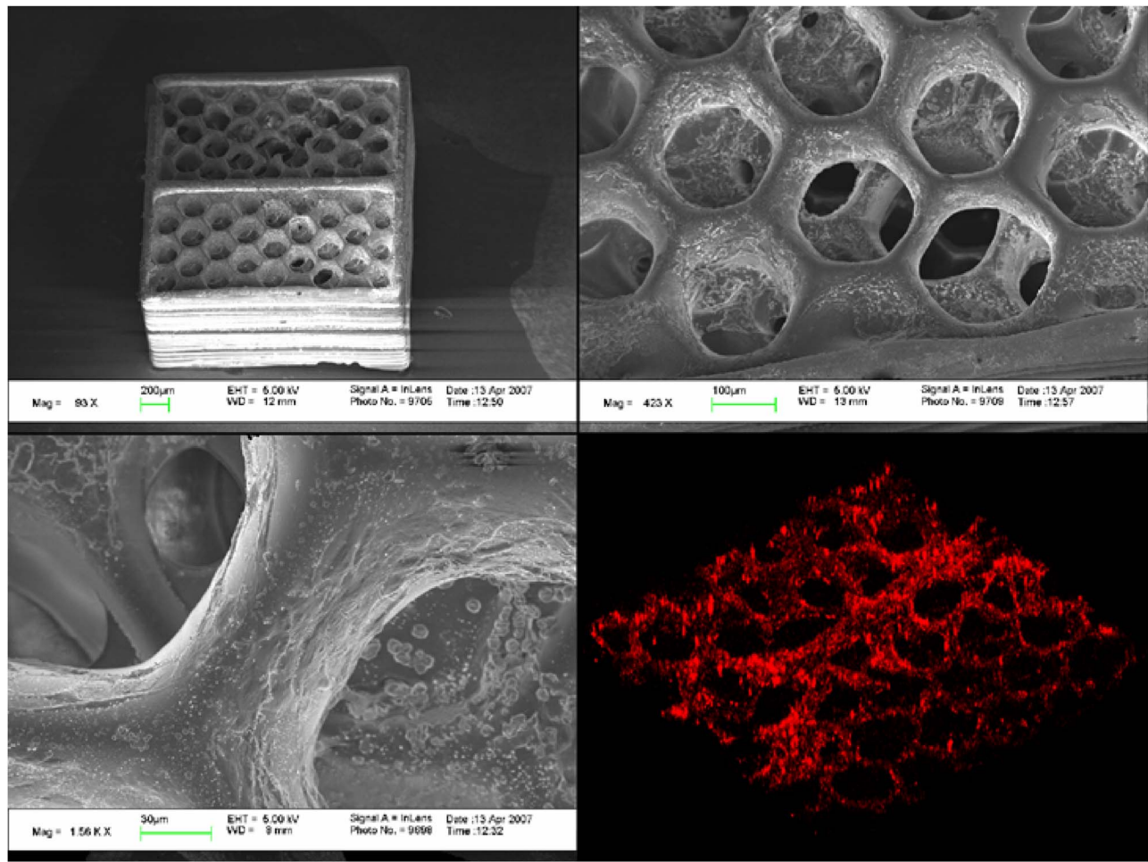
Fig. 3 Scanning electron micrographs in (A)–(C) depict a multilayered scaffold with interconnective, hexagonal-shaped porosity. An extracellular matrix secreted by attached D1 cells is visible in (C). D1 cells were stained with a fluorescent tracer dye prior to seeding onto fibronectin-modified scaffolds. (D) shows a reconstructed 3D image from fluorescence confocal microscopy, indicating that cells attached efficiently to the microfabricated scaffold.
