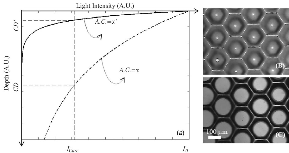
Fig. 1 The curing of monomer with and without the addition of the UV dye. (A) Theoretical model: The curing depth CD decreases when the absorption constant is increased after the addition of dye. (B) Photopatterning of PEGDA on a glass slide. The pores of a honeycomb structure are sealed by unwanted curing caused by scattered light. (C) Patterning the same monomer with the addition of UV dye Tinuvin 234 at a concentration of 0.2 wt %. The geometry of the honeycomb structure had increased feature resolution.
