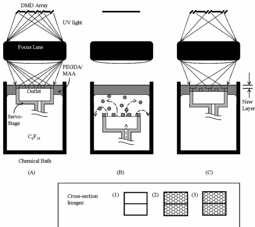
Fig. 2 The schematics of the DMD fabrication system showing the fabrication scheme (A)–(C) and the patterns of the scaffold cross section (inset)
