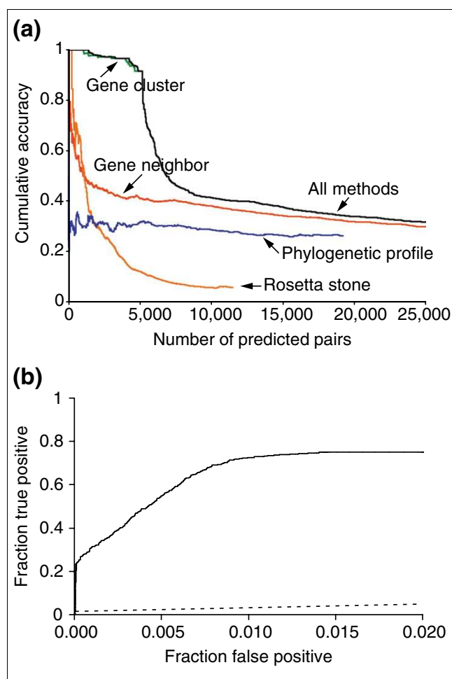
Figure 5 Assessment of the four methods by recovery of links between members of known E. coli protein complexes. (a) We test to see how often predicted interacting protein pairs are subunits of the same protein complex. E. coli protein complexes were obtained from the EcoCyc database. (b) Again, the ROC curve shows the performance of the rank-ordered list of all E. coli predicted interactions (solid line) compared with the random selection of protein pairs (dashed line), in their ability to recover constituents of known protein complexes.
