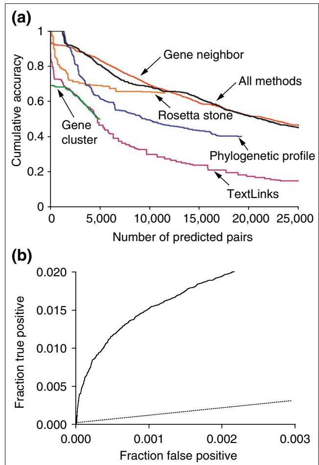
Figure 2 We assess COG category recovery for the four individual methods, the combination of the four methods, and TextLinks. (a) We assign a confidence measure to the likelihood that a pair of proteins is acting within the same COG pathway, reflecting the number of COG-annotated pairs that lie within the same pathway relative to the total number of annotated pairs. The COG confidence metric is used in the network-graphing function of the Proteome Navigator to select inferred protein linkages with uniform confidence. E. coli protein pairs displayed in this figure have a COG pathway confidence recovery (cumulative accuracy) of greater than 0.4, with the exception of the TextLinks pairs. (b) The receiver operator characteristic (ROC) curve shows the performance of the rank-ordered list of all E. coli interactions predicted from genomic inference (solid line) compared with the random selection of protein pairs (dashed line).
