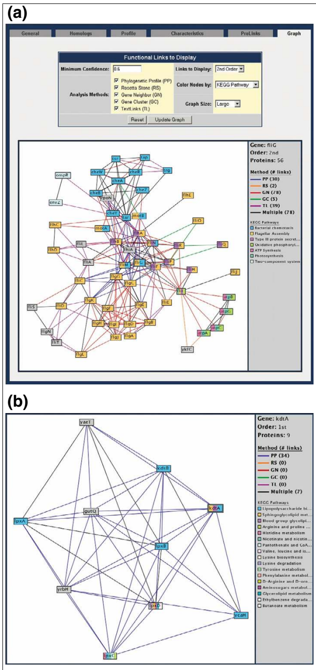
Figure 4 The 'Graphing' function of the Proteome Navigator displays the network of interactions satisfying the input search criterion. (a) Nodes are colored by functional categories explained in the right-hand border. Edges connecting proteins are colored by the method predicting the interaction, also described in the figure border. Associations predicted by multiple methods are shown in black. The double box around flIG indicates that this was the input protein used to generate this network. Clicking on a node brings the user to a protein-annotation page, and the search can be continued using the new protein to generate a new network search. (b) An example of functional discovery using Prolinks. Using kdtA as the initial seed, we speculate that GutQ, an uncharacterized E. coli protein, may be associated with lipopolysaccharide and cell-wall synthesis. Confirmation of these predictions awaits further scientific inquiry.
