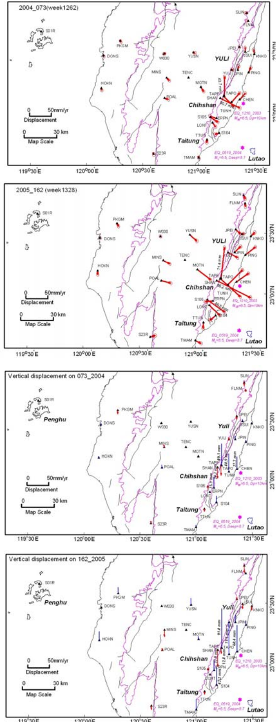
Figure 5. Poseismic displacements relative to Paisha, Penghu (S01R). The upper graph show the horizontal postseismic displacement in third and eighteenth month and the elevation changes in GPS height for the postseismic displacements (lower graph), respectively.
