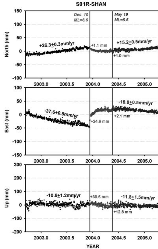
Figure 3. Position variation in station pairs, S01R-S104 (upper graph) and S01R-SHAN (lower graph). For each subplot, the abscissa denotes the time in year, and the ordinate are the north, east and up components of each baseline, respectively. The vertical line in each subplot indicates the time of the earthquakes, the number with the uncertainty values of the line express the relative velocities and the numbers without the uncertainty value means the relative coseismic displacements of the earthquake.
