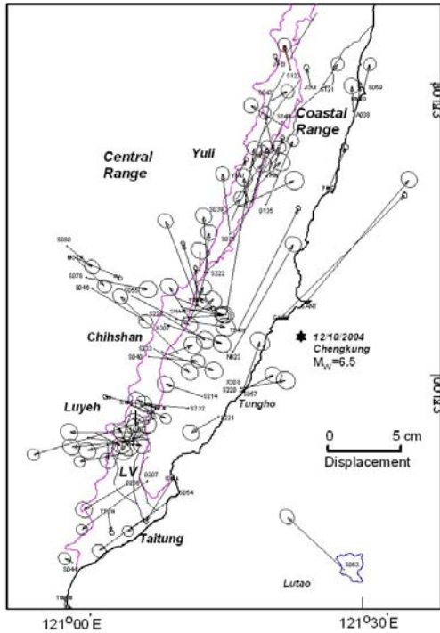
Figure 1. Horizontal coseismic displacements relative to Paisha, Penghu. The 95% confidence error ellipse is shown at the tip of each coseismic vector. The epicenter is marked by a solid star. LV and LVF denote the Longitudinal Valley and Lngitudinal Valley Fault, respectively
