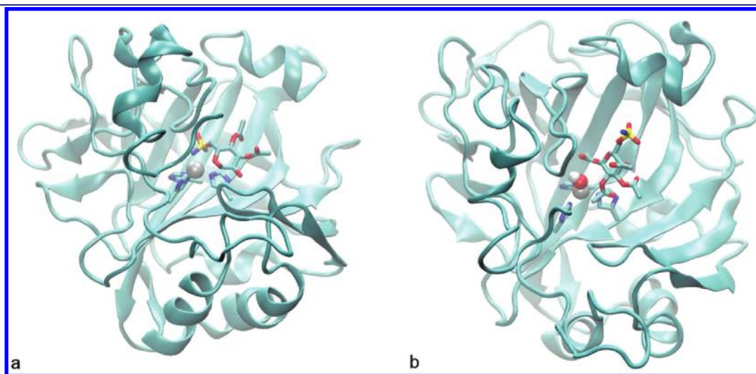
Figure 6. Active site structure of hCA II with the ligand inside the pocket. (a) Pure inhibitor conformation of compound 4 (X-ray structure CA II: 1b_4 ) and (b) substrate conformation of the parent sulfamate 1b (docking structure). Highlighted are the zinc (gray sphere), hydroxide (red-white spheres), ligand (licorice), and histidine residues (licorice in the background).
