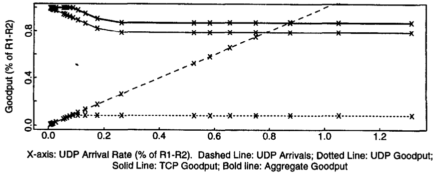
Fig. 5. Simulations with three TCP flows and one UDP flow, with WRR scheduling. There is no congestion collapse.
