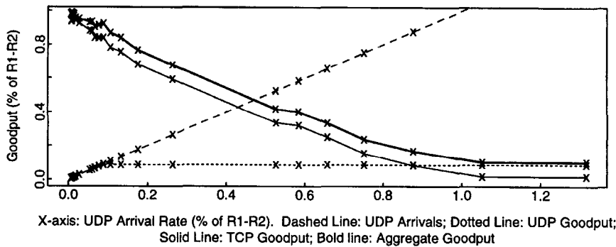
Fig. 6. Simulations with one TCP flow and three UDP flows, showing congestion collapse with FCFS scheduling.
