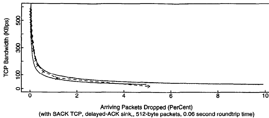
Fig. 11. TCP bandwidth versus steady-state drop rate, for SACK TCP with a delayed-ACK receiver, a 60-ms round-trip time and 512-byte packets.
