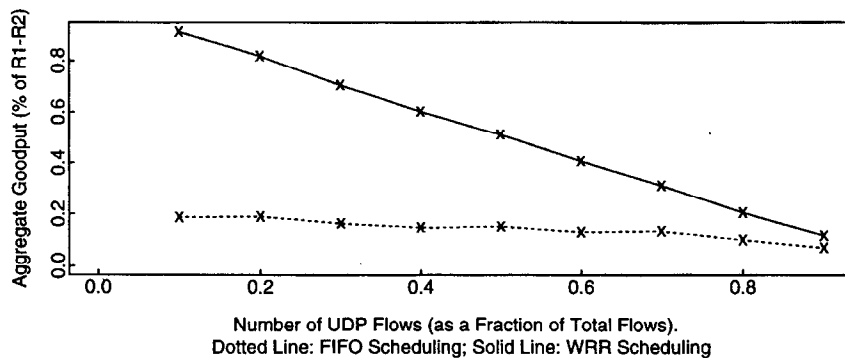
Fig. 8. Congestion collapse as the number of UDP flows increases.
