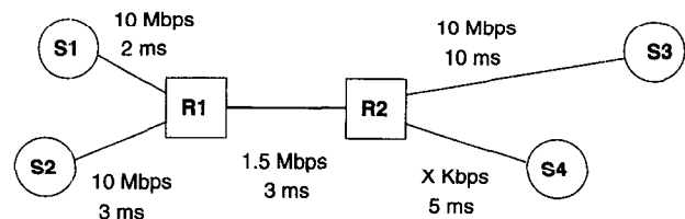
Fig. 1. Simulation network.
