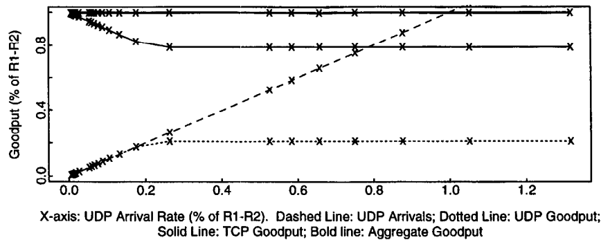
Fig. 3. Simulations with three TCP flows and one UDP flow, with WRR scheduling. There is no unfairness.
