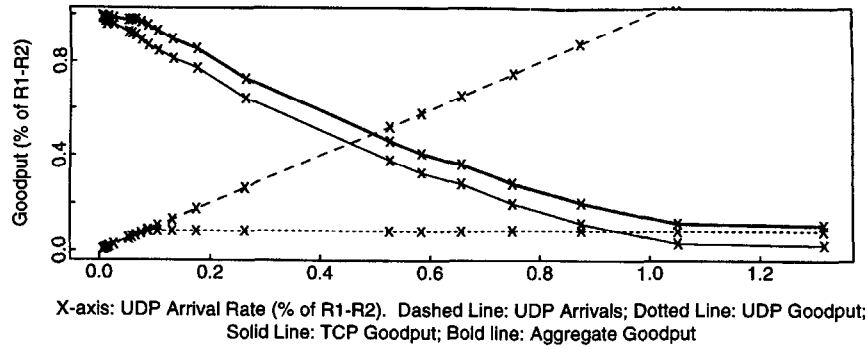
Fig. 4. Simulations showing congestion collapse with three TCP flows and one UDP flow, with FCFS scheduling.
