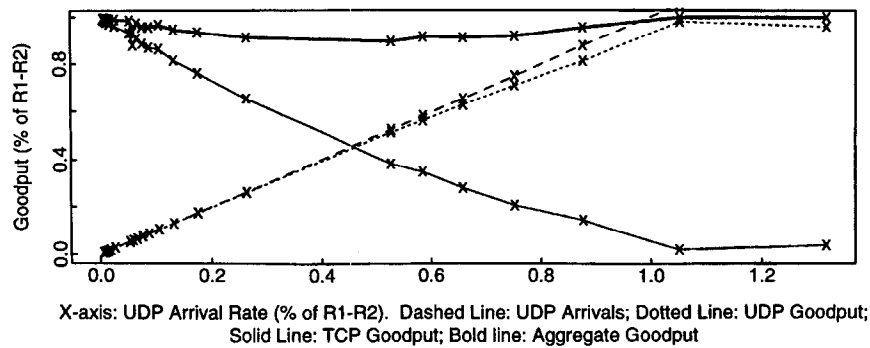
Fig. 2. Simulations showing extreme unfairness with three TCP flows and one UDP flow, with FCFS scheduling.
