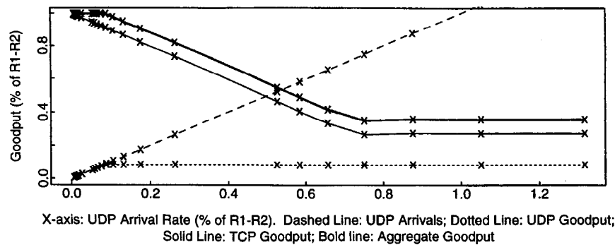
Fig. 7. Simulations with one TCP flow and three UDP flows, showing congestion collapse with WRR scheduling.
