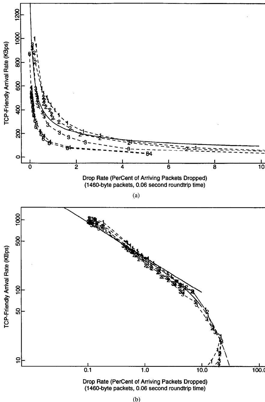
Fig. 10. TCP-friendly bandwidth for a 60-ms round-trip time and 1460-byte packets.
