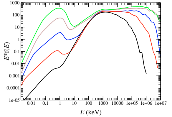
Fig. 2. Resulting spectrum (in the central engine frame) for different baryon loadings of the flow. From bottom to top the curves correspond to magnetization \sigma_0 = 40, 50, 60, 70, 100 (or corresponding baryon loading \eta \approx 250, 350, 460, 590, 1000 ) respectively. The high \sigma_0 flows are characterized broader spectra. The model predicts that bright prompt optical and UV emission is accompanied by powerful \sim GeV emission. For bright optical emission, the optical spectrum is expected to be hard.
