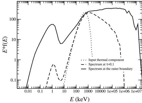
Fig. 1. Photon spectrum at different radii (or corresponding Thomson optical depths) in the flow. The spectrum is shown in the central engine frame. The dotted line stands for the spectrum at the radius where radiation and electrons decouple. The photospheric emission is shown with the dashed line (see also G06; GS07). The overall spectrum (solid line) includes the emission from the Thomson thin region of the flow. Synchrotron-self-absorbed emission from this region dominates the spectrum below \sim 10 keV. Inverse Compton leads to flat \gamma -ray tail up to \sim 1 GeV.
