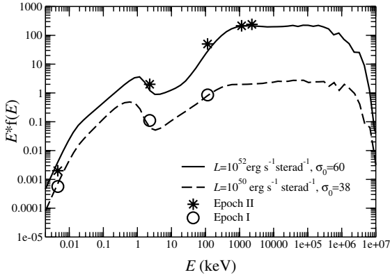
Fig. 3. Applying the model to multi frequency observations of the prompt emission of GRB 061121 (see Fig. 11 in Page et al. 2007). The circles stand for the observations of epoch I (just before the main pulse of the burst) and the stars for those of epoch II (during the pulse). Observations are blue-shifted by 1+z to the burst rest frame ( z = 1.131 for GRB 061121). The solid and dashed curves show spectra for two different sets of the parameters of the flow that illustrate that the model can account for the broad-band prompt spectra.
