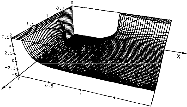
Figure 1. Tridimensional plot of the normalized potential
