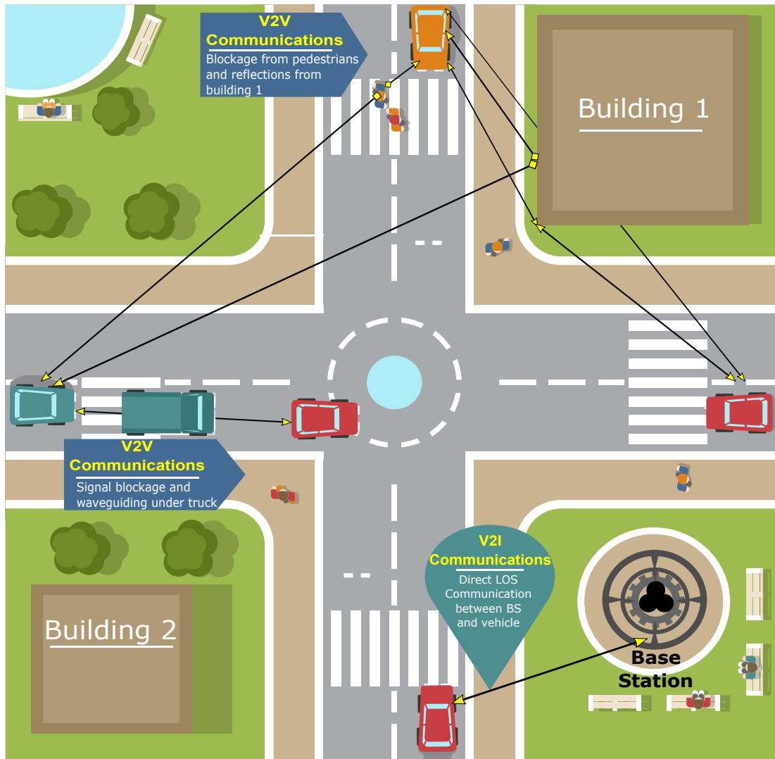
Fig. 2: Typical propagation effects and link types in mmWave vehicular communications.
