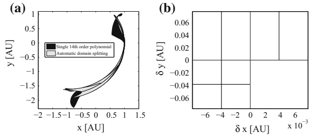
Fig. 7 Propagation of the initial uncertainty set in the two-body dynamics to t_i = 34.85 with automatic domain splitting.
