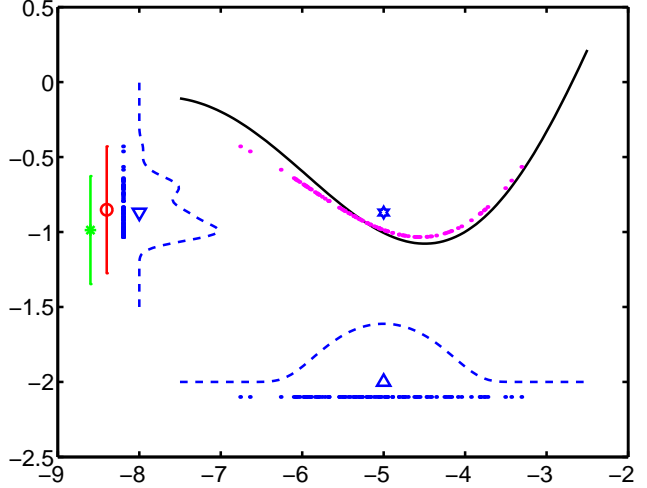
Fig. 1. Prediction with uncertain input. On the x-axis , the dashed line represents the Gaussian input distribution, with mean located by the triangle, from which we draw 100 samples (dots under it). In the middle of the figure , the solid line represents the true underlying function. We fit a model to it, and propagate the 100 input samples through the model (dots close to the true function). On the y-axis we project the 100 predicted values (dots) and use them to estimate the predictive density (dashed line), with mean located by the triangle. The error bar with a circle and the error bar with a star show the mean and 95% confidence interval of the Gaussian approximation with exact computation of mean and variance and of the method with Taylor expansion respectively.
