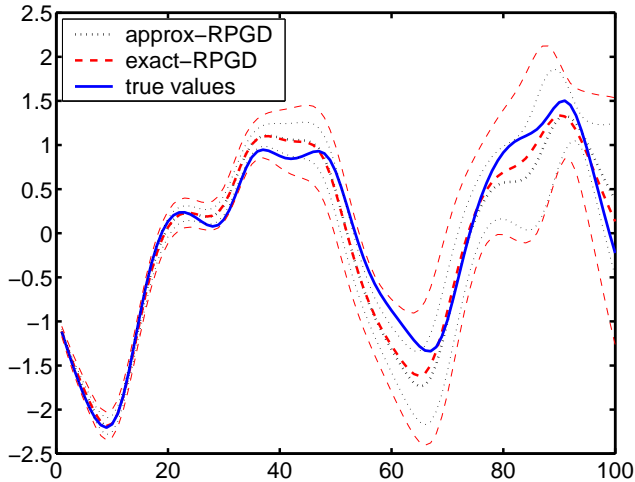
Fig. 2. 100 iterated predictions for the exact-RPGD (dashed) and approximate-RPGD (dotted): for each the thicker lines represent the mean of the predictive distributions and the two thinner lines around represent the upper and lower bounds of the 95% confidence interval of the Gaussian predictive distributions. The solid line shows the true target values.
