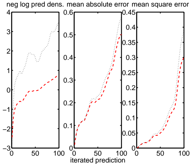
Fig. 3. Negative log predictive density, mean absolute error and mean squared error as a function of the iterative prediction horizon for the exact-RPGD method (dashed) and for the approximate-RPGD (dotted). Averages over 200 repetitions.
