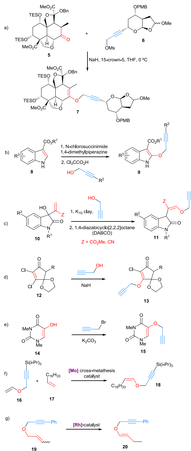
Scheme 8. Miscellaneous synthesis of propargyl vinyl ethers.
