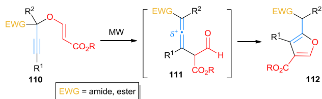
Scheme 29. Metal-free, microwave-induced synthesis of furans.
