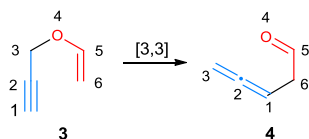
Propargyl vinyl rearrangement
