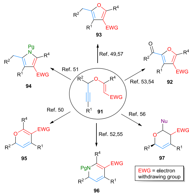
Scheme 25. Metal-catalysed transformations from PVEs.
