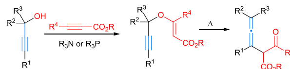
Scheme 7. Synthesis from propargyl alcohols and conjugated alkynoates.
