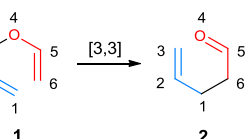
Allyl vinyl rearrangement
