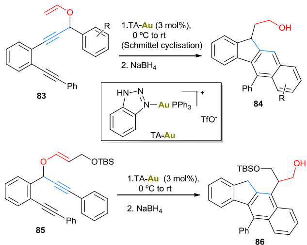
Scheme 23. Gold-catalysed propargyl Claisen rearrangement – Schmittl cyclisation.
