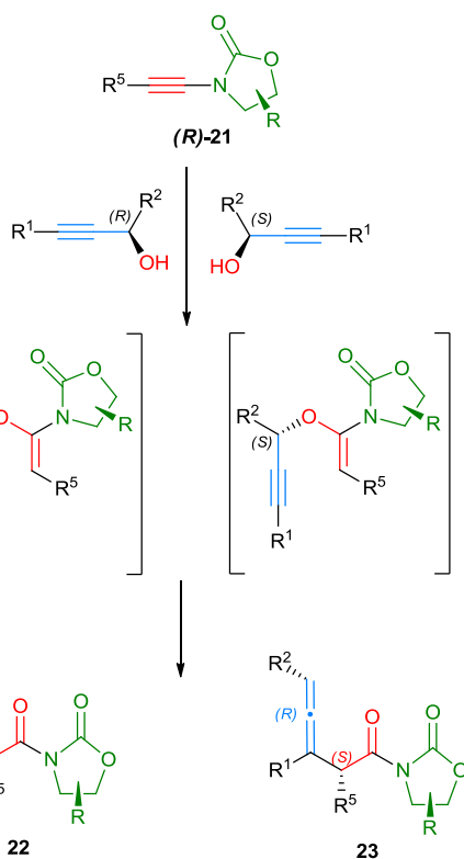
Scheme 9. Stereoselective propargyl Claisen rearrangement using chiral ynamides.
