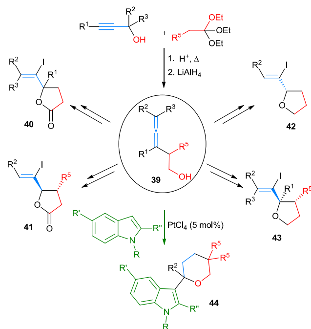
Scheme 13. Synthesis and applications of functionalised allenols 39 .
