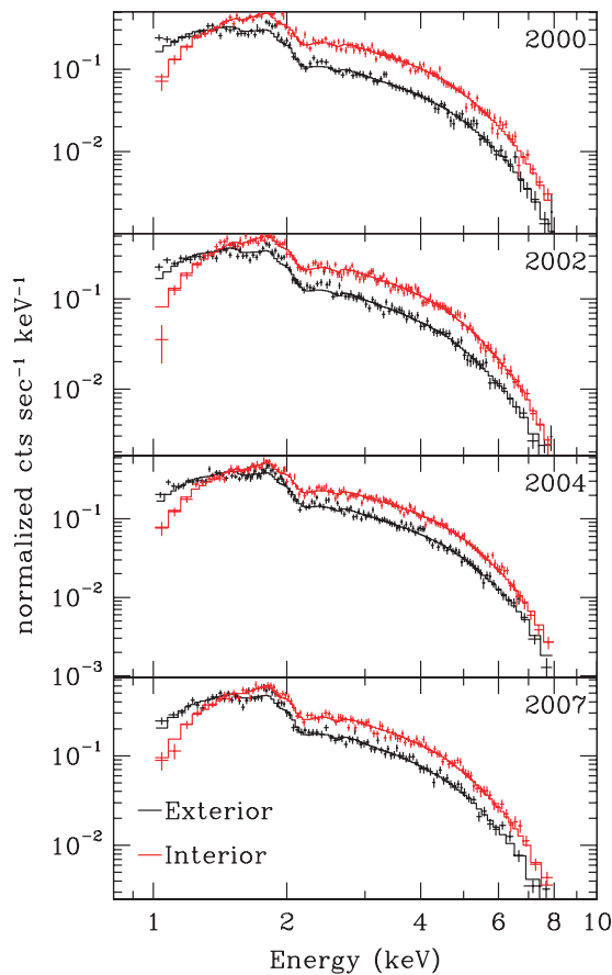
Figure 6. Extracted spectra for forward shock and interior nonthermal filaments. (A color version of this figure is available in the online journal.)
