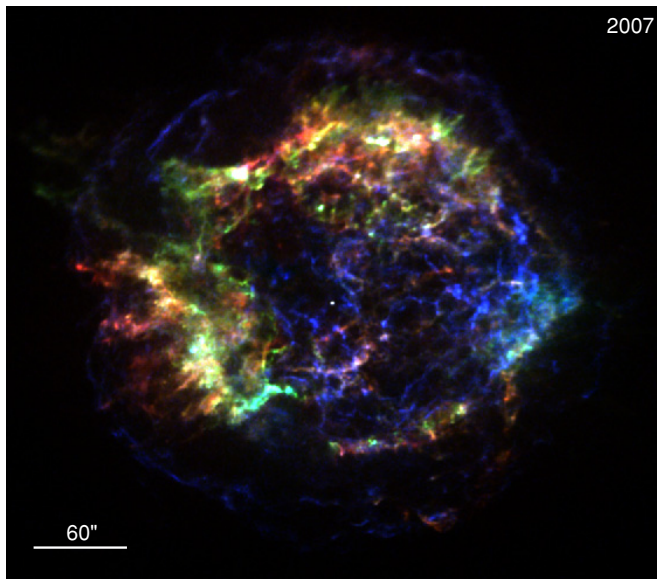
Figure 1. Exposure-corrected RGB color 2007 December image of Cas A. Red corresponds to 0.5–1.5 keV, green to 1.5–3.0 keV, and blue to 4.0–6.0 keV. This figure is part of the on-line animation, which shows the dynamical and spectral evolution of Cassiopeia A from 2000 January to 2007 December.
