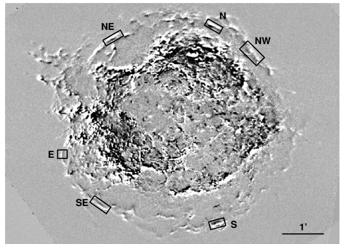
Figure 2. Difference image between 2000.08 and 2007.95 Chandra ACIS images. White correlates with the direction of filament motion. The boxes correspond to regions where we measured the filament proper motion.
