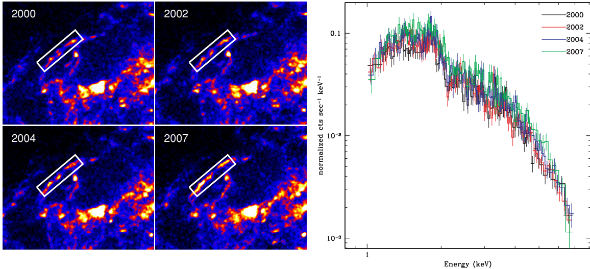
Figure 5. Left: exposure-corrected 4.2–6.0 keV images of a bright nonthermal filament (enclosed in the white box) in the northeast corner of Cas A. Right: spectral fits the spectrum from this filament. The fit results are listed in Table 3.
