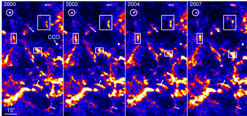
Figure 4. East-central region of Cas A in the 4.2–6.0 keV band. The four frames show the central region between 2000 and 2007. Boxes and the circle mark knots and filaments which show brightness variations along the filament, while arrows mark the location and direction of thin filaments which show proper motions between 2000 and 2007. The central compact object (CCO) is labeled for reference.
