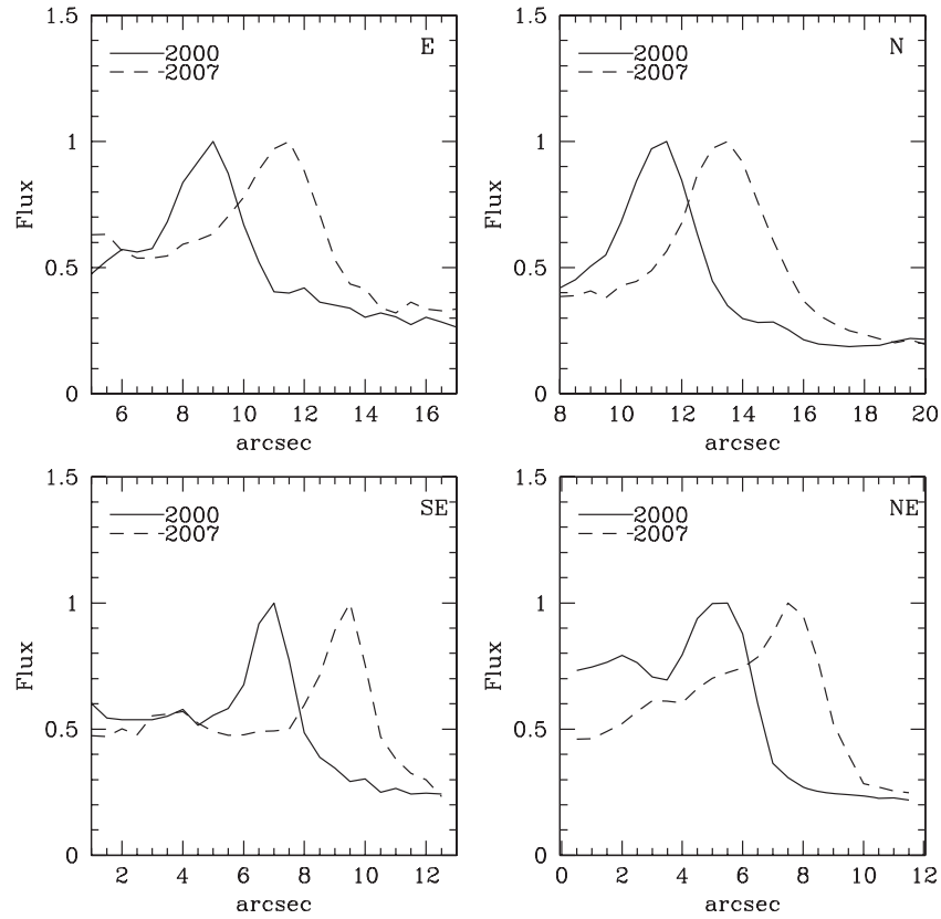
Figure 3. Nonthermal, forward shock filament emission profile plots are shown for four selected regions. Filament profiles from 2000 January and 2007 December are shown as solid and dashed lines, respectively.
