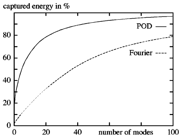
FIG. 7. Comparison of POD and Fourier-modes: captured fluctuating energy.
