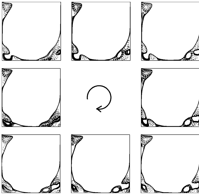
FIG. 22. Streaklines of one period of the periodic solution of the 80-dimensional system at Re = 11,800 . Solid lines indicate a clockwise rotation, and dashed lines indicate counter-clockwise rotation (compare Fig. 5).
