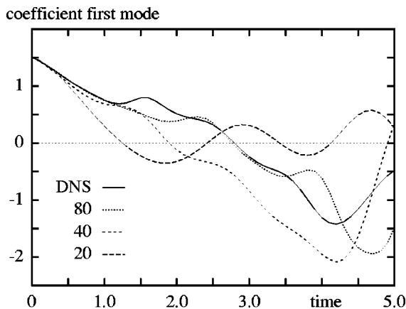
FIG. 13. The projection of the solution on the first eigenfunction \sigma_1 during one large-eddy turnover-time.
