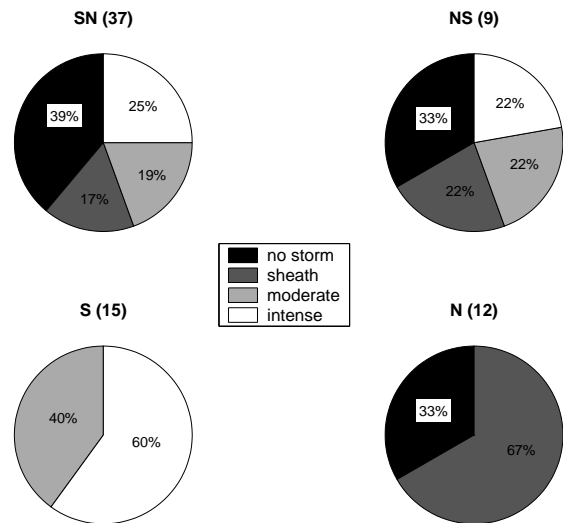
Fig. 14. The effect of the flux rope type to the geoeffectivity. Numbers in the parentheses show the total numbers of MCs identified in each category. Different colors demonstrate the different geomagnetic response: no storm at all, D_{st} > -50 nT (black); sheath region generated a storm (dark gray); MC caused a moderate storm (light gray); MC caused an intense storm (white).
