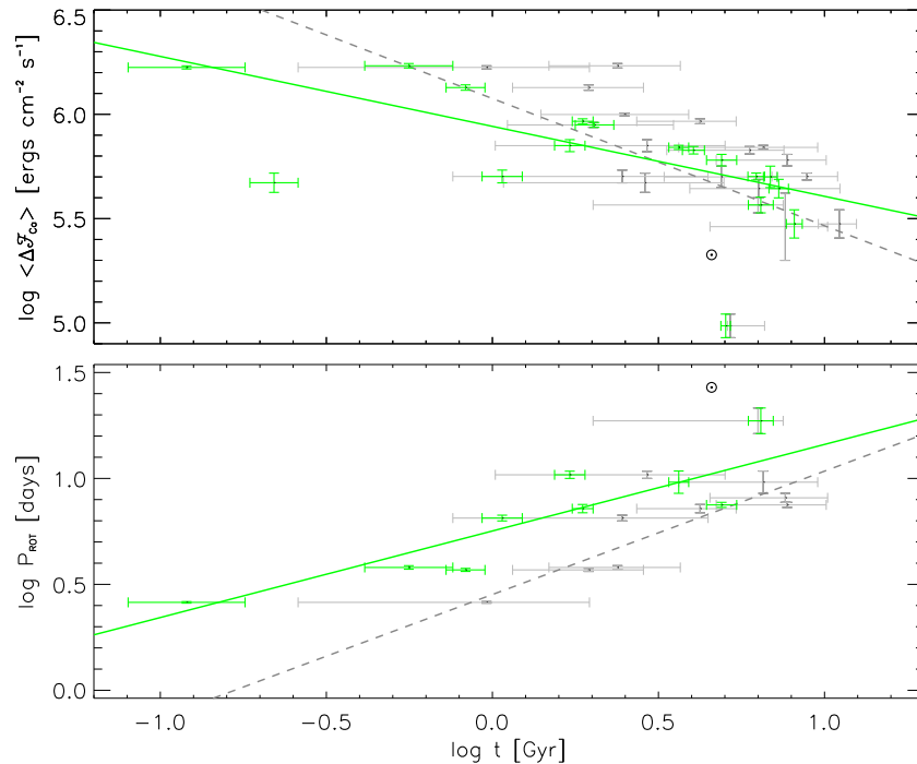
Figure 7. Age-activity (top; \chi_R^2 = 247 ) and age-rotation (bottom; \chi_R^2 = 38 ) relations from the Karoff et al. (2013) sample, using the original ages from SEEK (gray, dashed line) and the updated ages from AMP (green, solid line). Note that only SEEK results are shown for KIC 4914923, which is not included in our sample. The position of the Sun is indicated by the \odot symbol.
