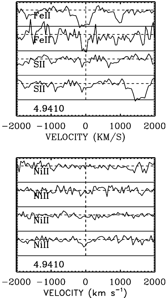
FIG. 3.—Upper panel, bottom to top: Lines S II \lambda 1251 , S II \lambda 1254 , Fe II \lambda 1608 , and Fe II \lambda 1260 . Lower panel, bottom to top: Lines Ni II \lambda 1317 , Ni II \lambda 1370 , Ni II \lambda 1455 , and Ni II \lambda 1467 . For each species, the lines are shown in order of decreasing oscillator strength, with the stronger lines at the bottom and the weaker at the top. The higher noise at Fe 1608 Å is a result of decreasing throughput at longer wavelengths.
