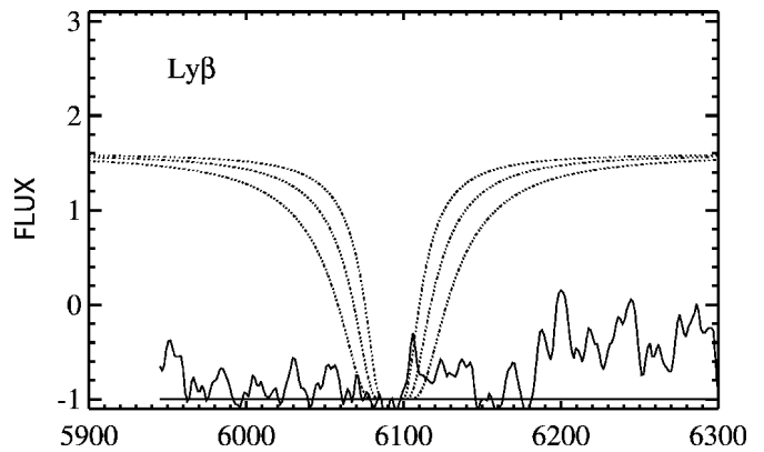
FIG. 2.—Damped \text{Ly}\alpha and \text{L}\beta profiles for N(\text{H I}) of 1 \times 10^{21} , 2 \times 10^{21} , and 4 \times 10^{21} \text{ cm}^{-2} .
