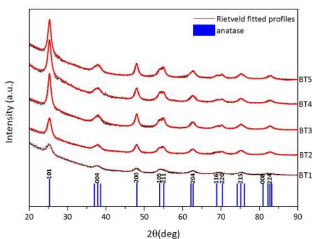
Figure 2. XRD patterns of TiO 2 (B)
