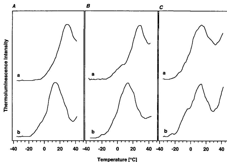
Fig. 5 Thermoluminescence glow curves of thylakoids from wild-type C. reinhardtii (A), His-tagged thylakoids from D2-H cells (B) and His-tagged PSII core complex (C) isolated from D2-H cells. Samples were illuminated with a single flash given at -10^{\circ}\text{C} in the absence (traces a) and presence (traces b) of 10\ \mu\text{M} DCMU, and glow curves were recorded at a heating rate of \sim 1^{\circ}\text{C s}^{-1} .
