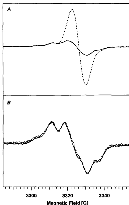
Fig. 4 EPR spectra of His-tagged thylakoids (A) and His-tagged PSII core complex (B) isolated from C. reinhardtii D2-H cells. The dotted- and the solid-curves indicate spectra measured in the presence and absence of 5 mM ferricyanide, respectively. Chl concentrations of thylakoids and isolated PSII core complex were 3 \text{ mg} and 0.6 \text{ mg Chl ml}^{-1} , respectively. Measuring conditions were as follows: microwave frequency, 9.3 GHz; microwave power, 0.05 mW; modulation frequency, 100 kHz; field modulation, 5 G; time constant, 0.3; scan time, 2 min; gain, 1 \times 10^3 .
