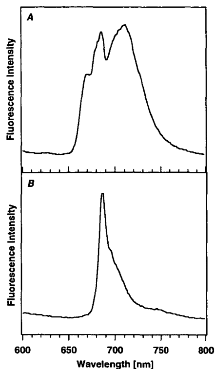
Fig. 3 77 K fluorescence emission spectra of His-tagged thylakoids (A) and His-tagged PSII core complex (B) isolated from C. reinhardtii D2-H cells. Chl concentrations were 0.4 \mu\text{g} and 0.2 \mu\text{g Chl ml}^{-1} for (A) and (B), respectively. Excitation wavelength was 435 nm.
