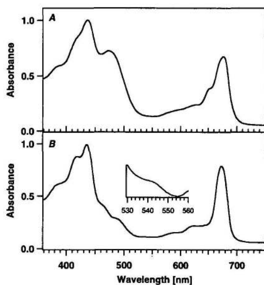
Fig. 1 Room temperature absorption spectra of His-tagged thylakoids (A) and His-tagged PSII core complex (B) isolated from C. reinhardtii D2-H cells. Inset in panel B: expanded spectrum in 530–560 nm region.
