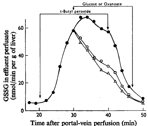
Fig. 9. Effects of glucose and octanoate on the rate of GSSG release in the perfused liver of starved rats
