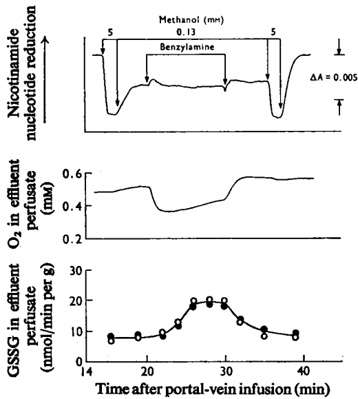
Fig. 11. Effects of benzylamine infusion on the steady state of the catalase H_2O_2 intermediate, the rate of O_2 consumption and the rate of GSSG release in perfused liver
