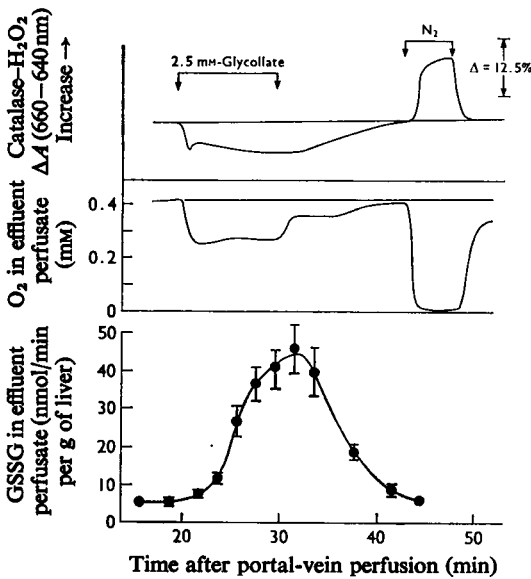
Fig. 6. GSSG release induced by glycollate oxidation in perfused liver
