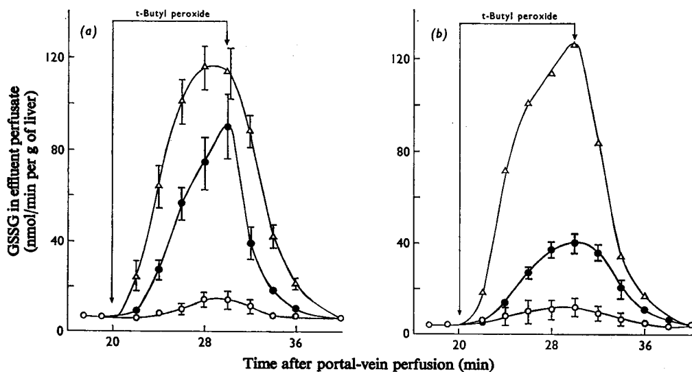
Fig. 8. Relationship between the rates of GSSG release and t-butyl hydroperoxide reduction by perfused liver under different metabolic conditions
