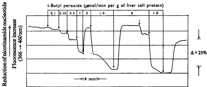
Fig. 2. Oxidation-reduction state of nicotinamide nucleotides in isolated liver cells during the reaction of glutathione peroxidase. Isolated liver cells at 5.1 mg of protein/ml were incubated with the medium used for the perfusion experiments. O 2 /CO 2 (19:1) was supplied constantly with magnetic stirring at 30°C. t-Butyl hydroperoxide was infused continuously into the suspension at the rates indicated on the Figure, and the fluorescence change of nicotinamide nucleotides was recorded at an emission wavelength of 460 nm, with excitation at 366 nm. Arrow on curve indicates the addition of pentachlorophenol (60 µM).
