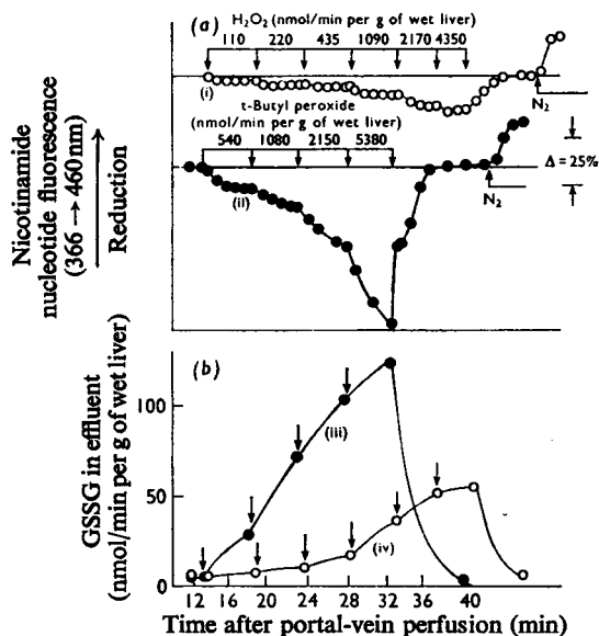
Fig. 1. Effect of H_2O_2 and t-butyl hydroperoxide on the oxidation-reduction state of nicotinamide nucleotide (a) and on the rate of GSSG release from the perfused liver (b)
