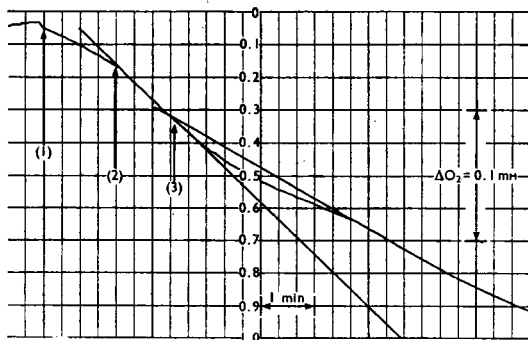
Fig. 12. Effect of t -butyl hydroperoxide on the respiration of isolated liver cells
