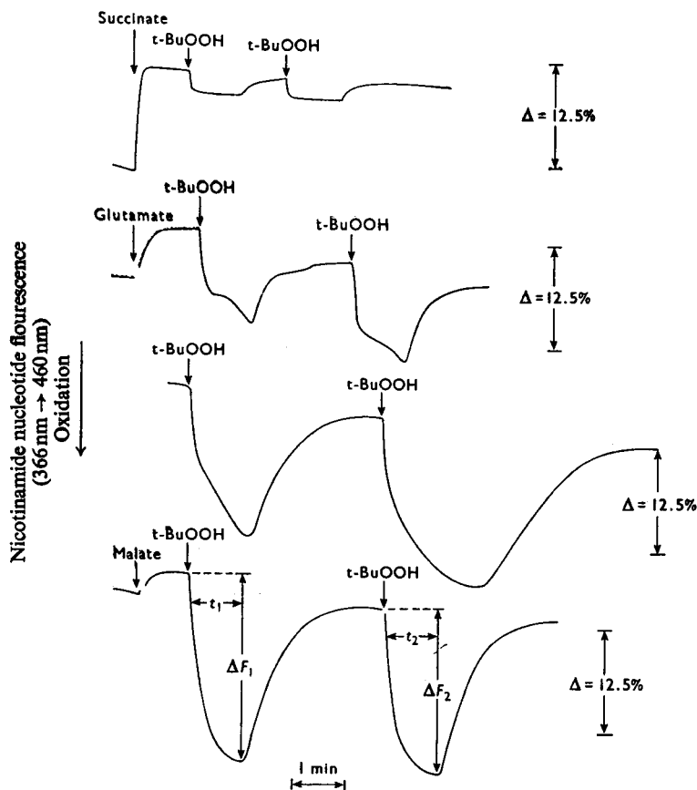
Fig. 5. Rate of hydroperoxide reduction by isolated mitochondria, and its effect on the redox state of nicotinamide nucleotides. The reaction mixture consisted of 225 mM-mannitol, 75 mM-sucrose, 0.1 mM-EDTA, 20 mM-Tris/HCl buffer, pH 7.4, 4 mM-potassium phosphate, pH 7.4, and rat liver mitochondria prepared as described in the text at a concentration of 7.1 mg of protein/ml. The oxidation and re-reduction of nicotinamide nucleotides caused by the addition of 0.15 mM-t-butyl hydroperoxide were measured fluorimetrically at 30°C; 5 mM-succinate, 5 mM-glutamate and 5 mM-malate (or -octanoate) were added as shown on the Figure. F represents the extent of fluorescence change in arbitrary units, and t the time required for consumption of the added t-butyl hydroperoxide.
