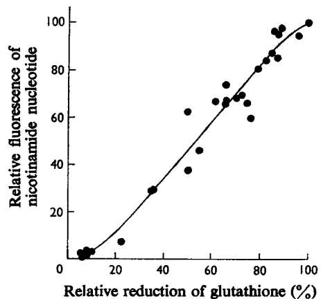
Fig. 3. Relative oxidation-reduction states of nicotinamide nucleotides and of glutathione in isolated liver cells during the reaction of glutathione peroxidase
