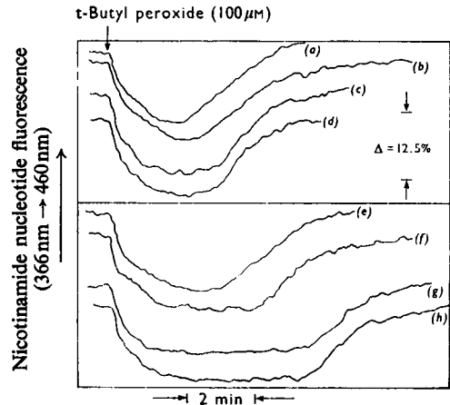
Fig. 4. Effects of various substances on the rate of t -butyl hydroperoxide reduction by isolated liver cells
