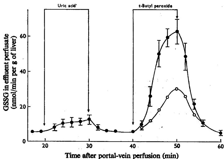
Fig. 10. GSSG release during oxidation of uric acid in the perfused liver of the aminotriazole-pretreated rat. The liver of the starved rat pretreated with 3-amino-1,2,4-triazole was perfused without exogenous substrates. Uric acid (1 mM) and t-butyl hydroperoxide at 362 nmol/min per g of liver (●) or 188 nmol/min per g of liver (○) ( n = 2 ) were infused for 10 min respectively, as indicated in the Figure. The rate of uric acid disappearance from the perfusate under these conditions was 600 \pm 40 nmol/min per g of liver and the rate of increased O_2 consumption was 418 \pm 27 nmol/min per g of liver. Each point is the mean value \pm s.e.m. of five separate experiments. Although the experimental values are not shown, the infusion of uric acid into the control rat liver did not stimulate any detectable increase in the GSSG release.
