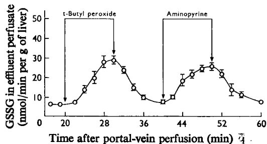
Fig. 7. GSSG release observed during demethylation of aminopyrine in the liver of phenobarbital-pretreated rats
