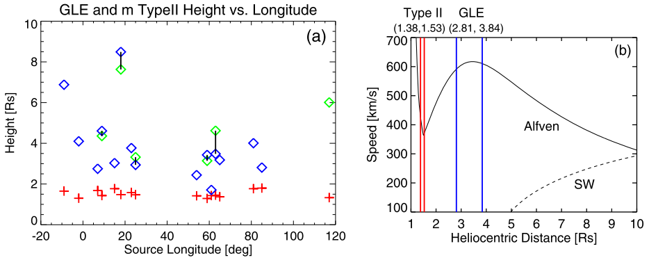
Fig. 16 (a) The CME heights at SPR ( diamonds ) and type II burst onset ('+' symbols). The green diamonds denote data points obtained from linear extrapolation of the LASCO CME height to the SPR time. The blue diamonds are data points obtained by quadratic extrapolation from the flare onset to SPR using the acceleration a_4 . Data points obtained by both methods are connected by the solid lines . (b) The average CME heights at SPR (minimum = 2.81 R_s ; maximum = 3.84 R_s ) and type II onset SPR (minimum = 1.38 R_s ; maximum = 1.53 R_s ) from Fig. 14 superposed on the Alfvén speed profile. The rise in solar wind speed (SW) is also shown for comparison
