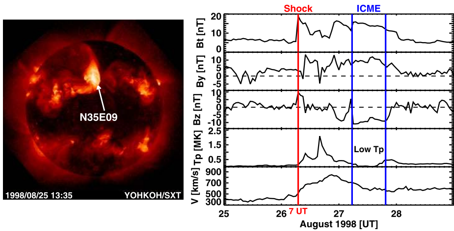
Fig. 3 (Left) Yohkoh/SXT image at 13:35 UT 1998 August 25 showing the post-eruption arcade from the source active region at N35E09. The flare occurred at 21:50 UT on 1998 August 24. (Right) In-situ measurements of solar wind magnetic field and plasma parameters showing the shock and ICME on 1998 August 26–27
