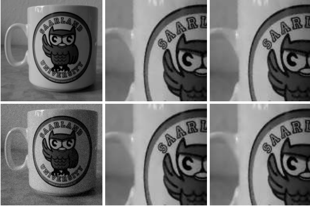
Figure 9: Denoising of for real-world data with Perona-Malik diffusivity g(s^2) = (1 + s^2/\lambda^2)^{-1} . Top left: Original image, 256 \times 256 pixels. Bottom left: With additive Gaussian noise, standard deviation \sigma = 10 . Top centre and right: Second order nonlinear diffusion. Bottom centre and right: Fourth order nonlinear diffusion. Middle column: Results with optimal \ell^1 -error. Right column: Results with optimal \ell^2 -error.
