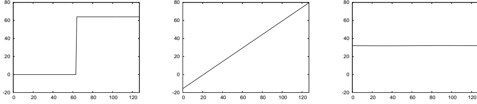
Figure 3: Stability of diffusion filtering and importance of boundary conditions. Left : Original signal, 128 pixels. Middle : Steady state of fourth order linear diffusion filtering with natural boundary conditions. Right : Same with periodic boundary conditions.
