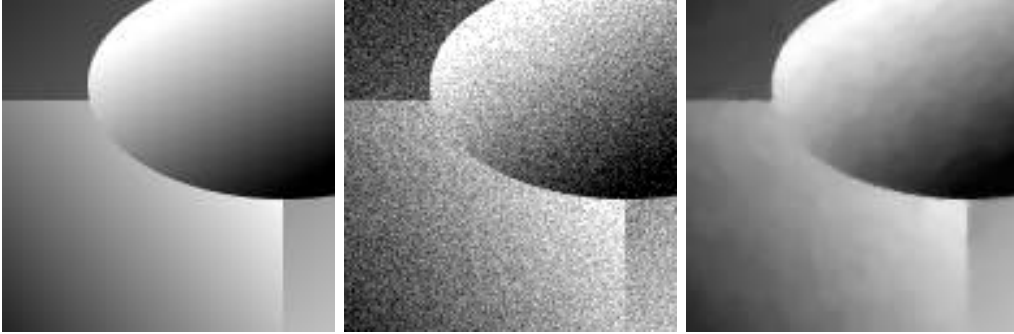
Figure 1: Left: Original image, 128 \times 128 pixels. Middle: With additive Gaussian noise, standard deviation \sigma = 20 . Right: Regularised total variation diffusion g(s^2) = (s^2 + \lambda^2)^{-1/2} with \lambda = 0.01 , stopping time t = 20.75 .
