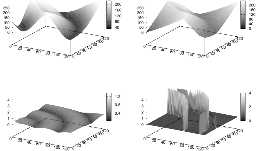
Figure 7: Fourth order Perona-Malik filtering and piecewise linearity. Top left: Original image, 128 \times 128 pixels. Top right: Fourth order Perona-Malik filtering. Bottom: Corresponding Frobenius norms of the Hessian.
