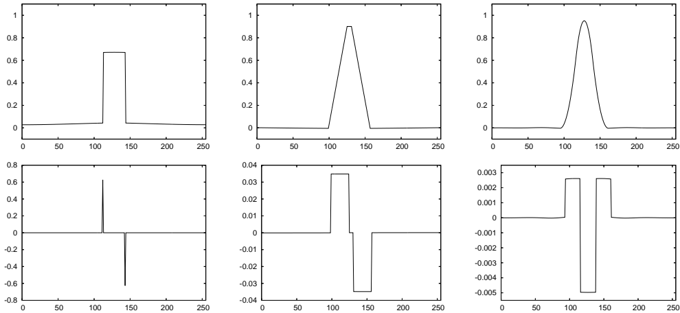
Figure 4: Perona-Malik filtering of a Gaussian kernel with different filtering orders. Top row : Filtering results for second, fourth and sixth order ( p = 1, 2, 3 ). Bottom left : First derivative of second order filtering result. Bottom middle : First derivative of fourth order filtering result. Bottom right : Second derivative of sixth order filtering result.
