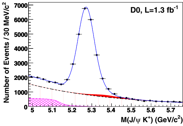
FIG. 1 (color online). Invariant mass distribution of J/\psi K^+ events. The solid line shows the sum of signal and background contributions, as described in the text. Shown separately are contributions from J/\psi\pi^+ events (solid filled area), J/\psi K^{*+} events (hatched area) and combinatorial background (dashed line).
