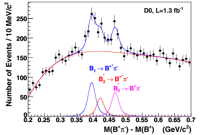
FIG. 2 (color online). Invariant mass difference \Delta M = M(B^+\pi^-) - M(B^+) for exclusive B decays. The line shows the fit described in the text. The contribution of background and the three signal peaks are shown separately.
