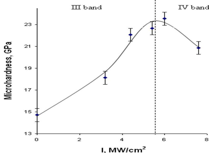
Figure 5 Microhardness of n -Si (111) wafer depending on laser intensity at load on indenter 20 g.
