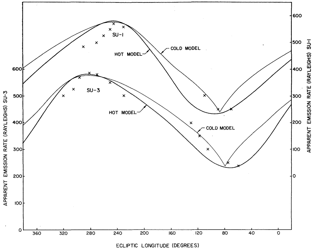
Figure 9 The comparison with the LASP data of the theoretical Lyman \alpha scattering intensity for the "cold" and "hot" models of the interstellar gas. The cold model contains an isotropic intensity of 240 R.
