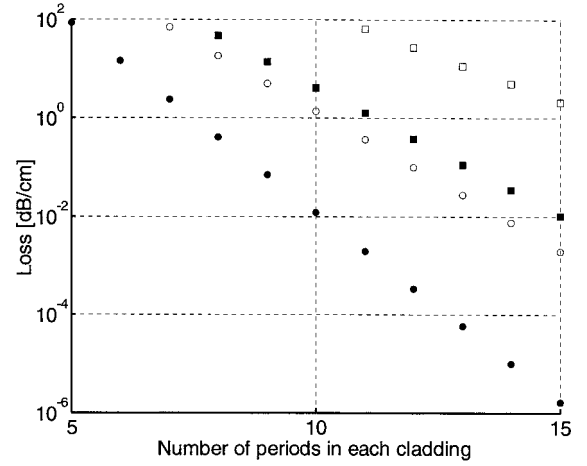
Fig. 3. Propagation loss in a QtW-BRW. Filled symbols, n_1 - n_2 = 0.5 ; open symbols, n_1 - n_2 = 0.4 . Circles, TE; squares, TM.
