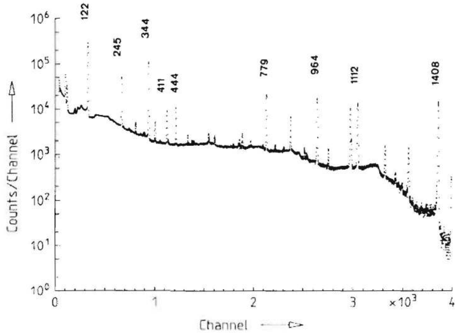
Figure 10.7: Pulse-height spectrum of ^{152}\text{Eu} . Energies in keV.
