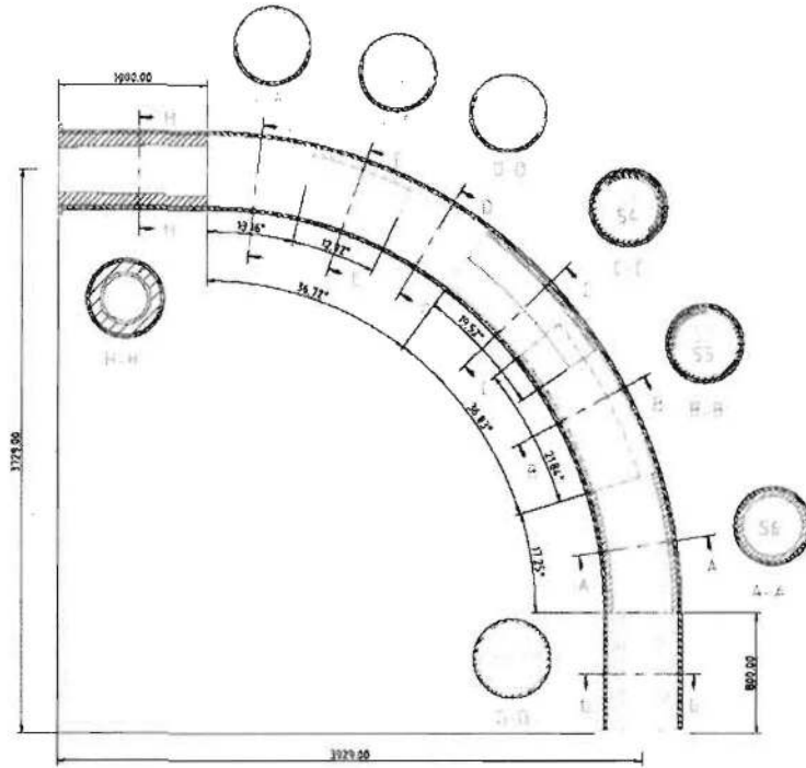
Figure 8.3: The first and second collimators (H and G) and the shielding to protect the TS coils (S).
