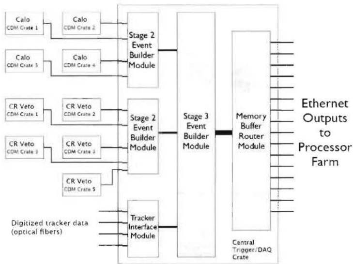
Figure 12.5: Schematic of the data flow in the Event Builder
