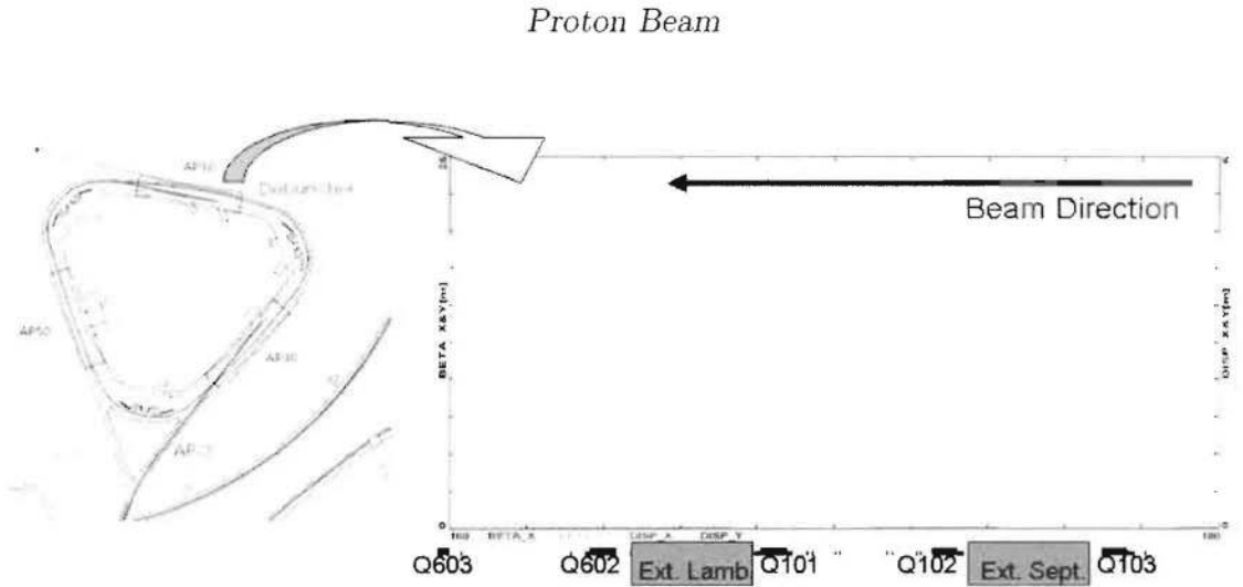
Figure 6.6: Proposed location for resonant extraction system. The electrostatic septum would be placed between quads Q103 and Q102 and the Lambertson would be placed between quads Q101 and Q602.
