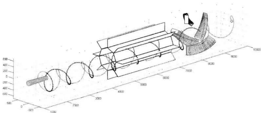
Figure 3.15: The path of a 105 MeV calibration electron fired from a cryomodule at the downstream end of the detector. Note the reconfiguration of the calorimeter.
