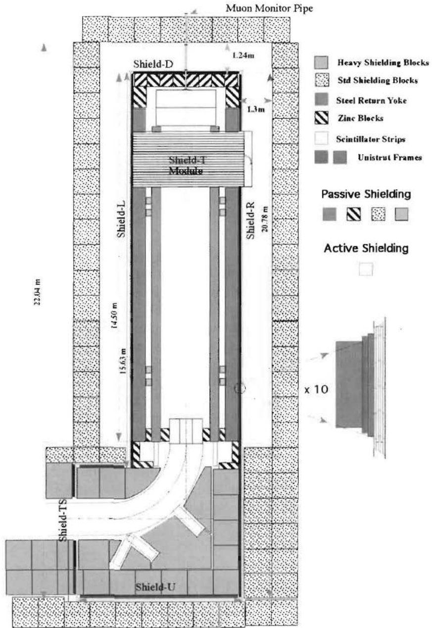
Figure 11.2: Top view of Cosmic Ray Shield
