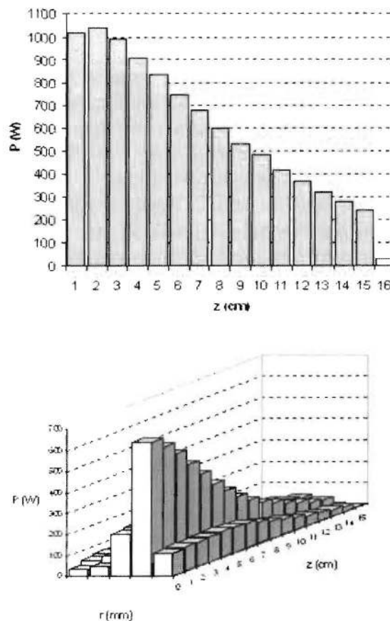
Figure 7.7: Pion production target power distributions with 3.0 mm radius and 16 cm length cylinder. These are the distributions used in cooling calculations, scaled to 9500 Watts total instantaneous power; the actual GEANT value is 7550 Watts.
