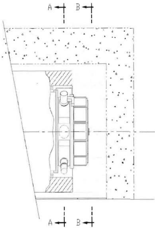
Figure 8.14: Vacuum closure two-piece configuration showing the VPSP with vacuum pumps and the IFB. The VPSP will remain attached to the solenoid while the IFB will be withdrawn during internal detector servicing.
