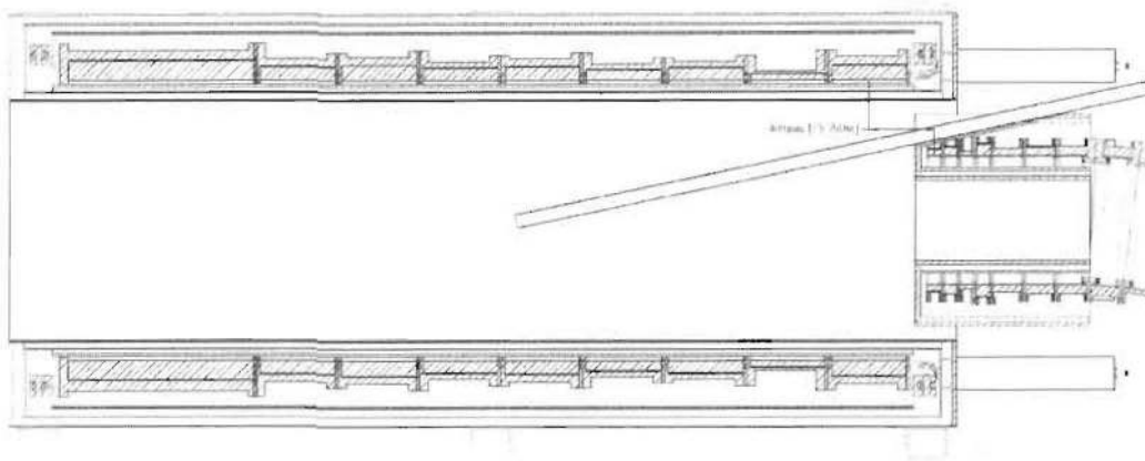
Figure 9.3: Proton beam interface. Proton beam enters the Mu2e apparatus between the coils of the PS and the TS.
