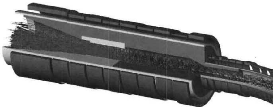
Figure 2.4: Cutaway view of the Production Solenoid. The initial proton beam enters the production solenoid from the right, and muons are collected and transported back to the right into the Transport Solenoid.
