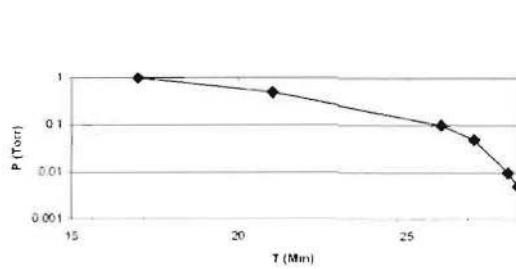
Figure 8.11: DS pressure during the initial pump-down. The cryopump gate valves are opened when the pressure is below 0.01 Torr.
