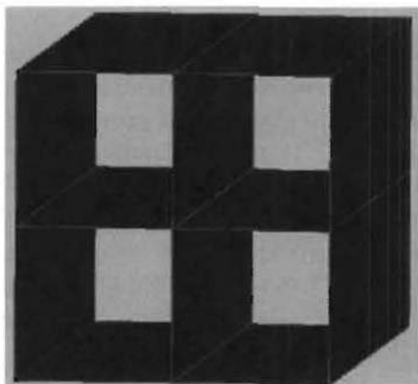
Figure 10.25: Carbon-epoxy square-cell honeycomb support for the \text{PbWO}_4 crystals.
