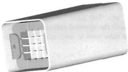
Figure 11.7: Isometric view of front of the H8711 PMT assembly. The Mu shield and 4x4 alignment grid are visible.
