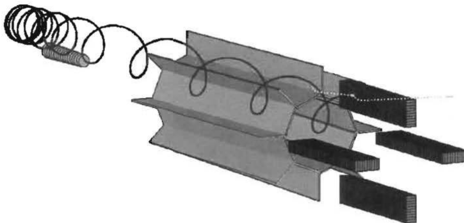
Figure 10.18: Isometric view of the Mu2e detector showing the straw tracker and the electromagnetic calorimeter, along with the track of a conversion electron.
