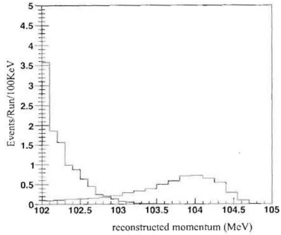
Figure 3.2: The final distribution of decay-in-orbit and signal events for a BR of 10^{-16} . The x -axis is the reconstructed momentum at the tracker.
