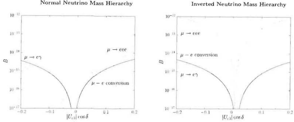
Figure 1.9: The branching ratios B for \mu \rightarrow e\gamma (solid line) and \mu \rightarrow eee (dashed line), and the normalized capture rate B for \mu \rightarrow e -conversion in Ti (dotted line) as a function of |U_{e3}| \cos \delta in a scenario where neutrino masses arise as a consequence of the presence of a triplet Higgs field with a small vacuum expectation value. The lightest neutrino mass is assumed to be negligible while the neutrino mass hierarchy is assumed to be normal (left-hand side) and inverted (right-hand side). See Ref. [38] for details.
