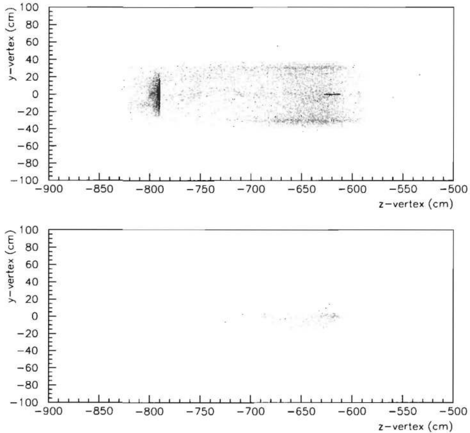
Figure 7.5: Distribution of positive (top) and negative (bottom) muon creation points in the Production Solenoid. Most positive muons are generated in the walls of the solenoid, surface muons, whereas negatives are largely from negative pion decay in flight.
