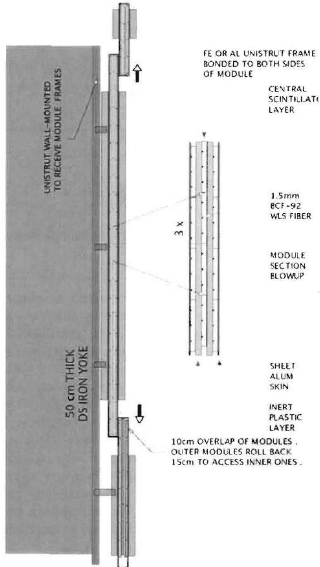
Figure 11.5: Sectional view of a full Cosmic Ray Shield module mounted to the Detector Solenoid return yoke
