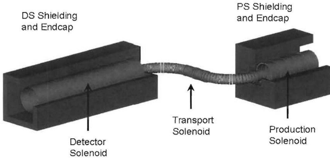
Figure 9.1: Sketch of the Mu2e magnetic elements showing the layout of the coils and the iron shielding.
