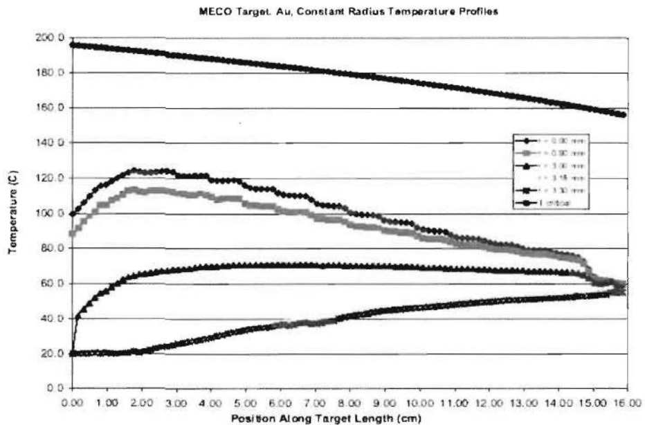
Figure 7.9: Target and coolant temperature at fixed radii as a function of position along the length. Our chief calculation tool has been CFDesign , a heat and mass transfer program designed for solving complex engineering problems. The results shown here are for a worst-case scenario, steady state heating, with power distribution shown in Fig. 7.7 and 9500 Watts total instantaneous power. Flow rate is 1 gallon per minute.
