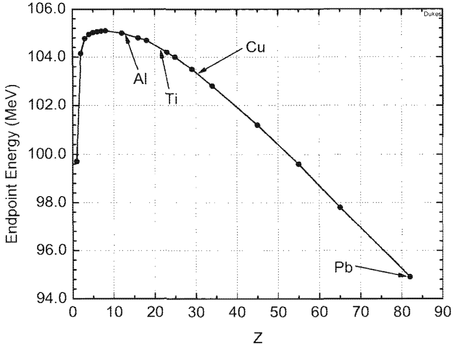
Figure 8.8: Muon decay-in-orbit endpoint energy vs atomic number.
