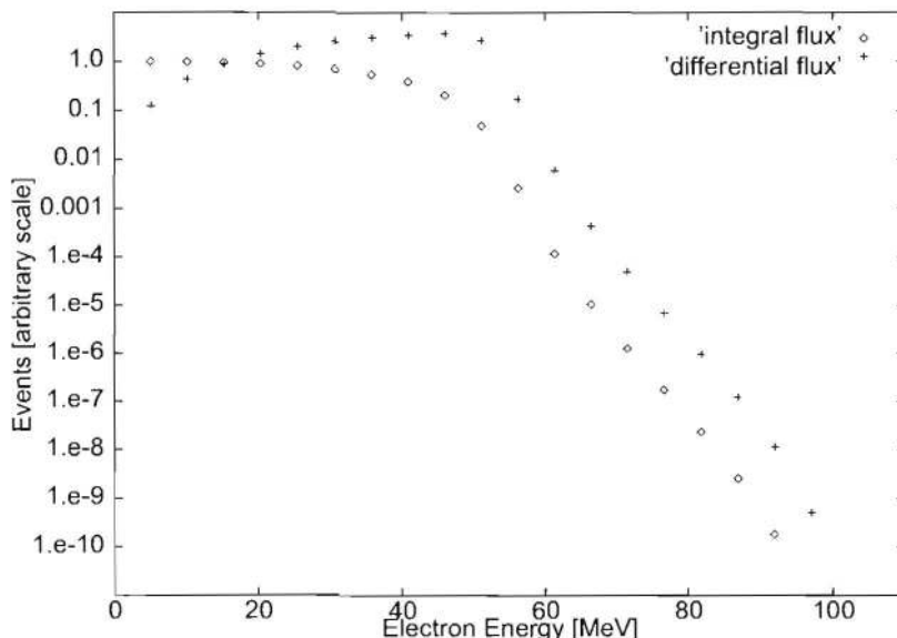
Figure 10.10: Plot of the differential and integral electron energy distributions for \mu decay in orbit. Circles are the integral of the distribution for energies above the abscissa value, and crosses are the differential distribution.
