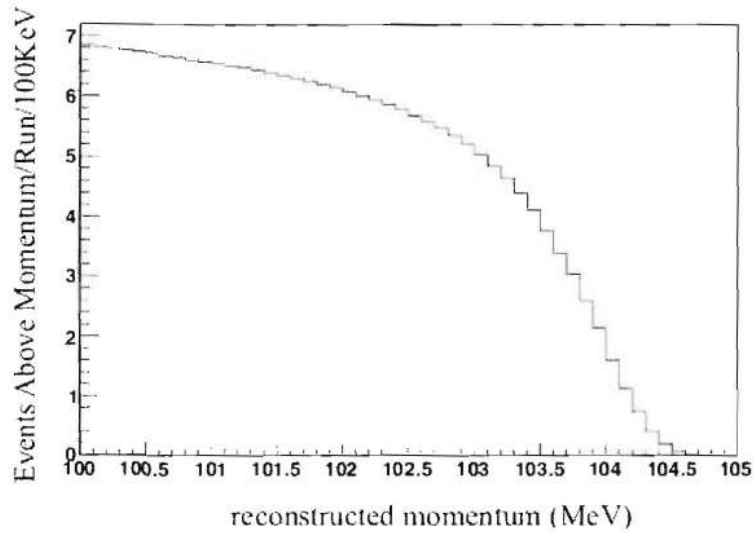
Figure 3.3: The integrated number of signal events above the indicated momentum at the tracker.
