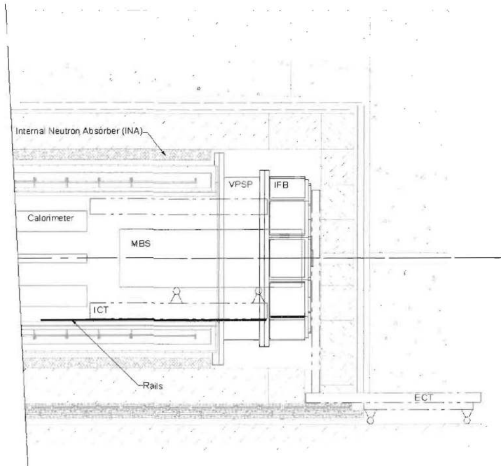
Figure 8.9: DS Vacuum Closure Elements. Note the Internal Neutron Absorber (INA), in green, that lies between the outer cryostat wall and the inner wall of the iron magnetic return yoke. It adds further protection to the active cosmic ray shield from slow neutrons from the DS. (The muon beam stop in this drawing is from an earlier design.)
