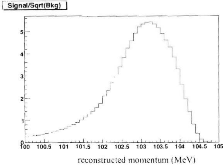
Figure 3.5: The quantity FOM = S/\sqrt{B} vs. lower cut on momentum, from the previous two plots, for a BR of 10^{-16} . We see for a cut at 103.25 MeV the FOM is maximized at 5.5.
