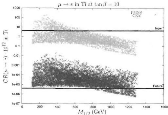
Figure 1.6: The \mu \rightarrow e conversion rate in Ti for different SUSY-GUT scenarios. The plots are obtained by scanning the LHC accessible parameter space. The horizontal lines are the present (SINDRUM II) bound and the planned (Future) sensitivity to the process both at the proposed PRIME experiment in JPARC and at the proposed Mu2e experiment at Fermilab. See Ref. [35] for details.
