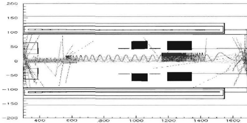
Figure 8.6: Trajectories of beam muons (green) and electrons (red) from muon decays. Blue indicates gammas, dashed black lines indicates neutrons. CH_2 is indicated by yellow lines.
