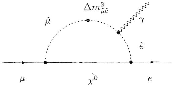
Figure 1.5: MSSM slepton-neutralino contribution to \mu \rightarrow e\gamma . \Delta m_{\tilde{\mu}e}^2 stands for the insertion of an off-diagonal element of the slepton mass-matrix. From [26].
