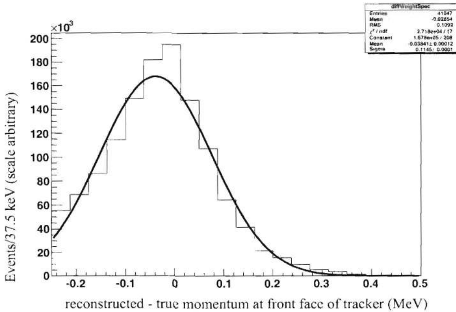
Figure 3.12: We examine decay-in-orbit events with an initial momentum at the foil greater than 90 MeV to gain in statistics. Here we take the side where decay in orbit events could smear into the signal and fit to a Gaussian, showing a resolution of 115 keV.
