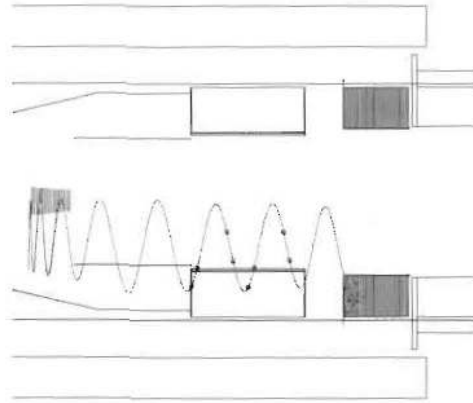
Figure 10.12: Simulated conversion electron trajectory.
