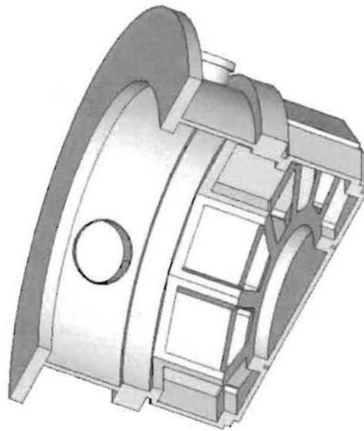
Figure 8.15: Perspective drawing of the IFB showing the facet covers and the wedge covers.
