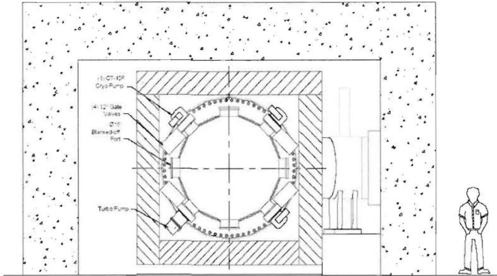
Figure 8.10: showing the three cryo vacuum pumps, one turbo pump, and four spare ports.
