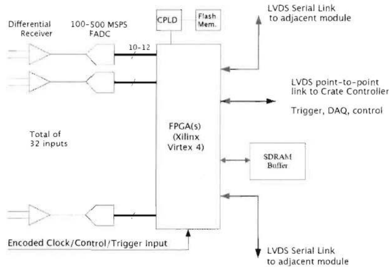
Figure 12.3: A block diagram of the Calorimeter Digitizer Module.
