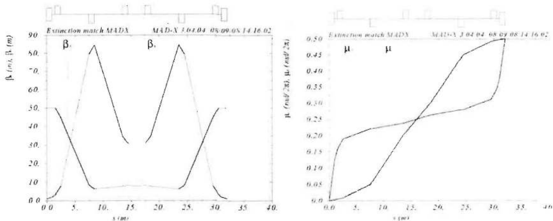
Figure 6.9: Preliminary extinction channel design.
