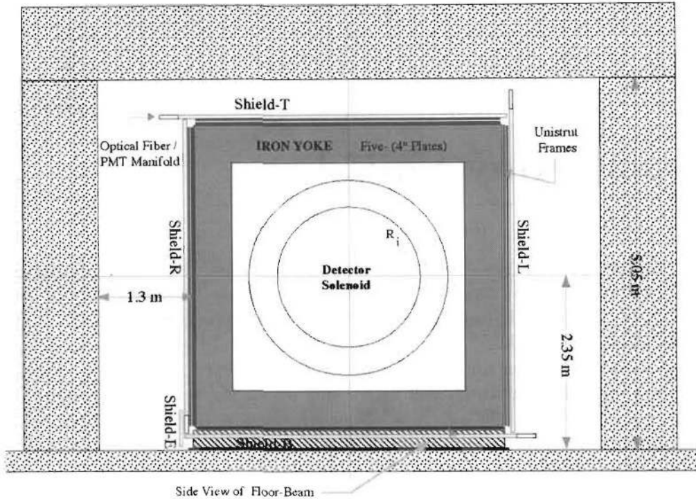
Figure 11.1: End view of Cosmic Ray Shield
