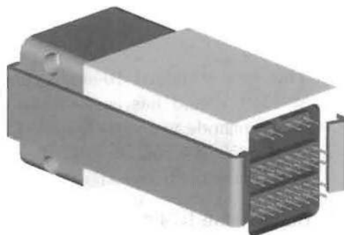
Figure 11.8: Isometric view of back of H8711 PMT assembly (without Mu shield). The pin connections for the 16 anodes and metal clip are shown.
