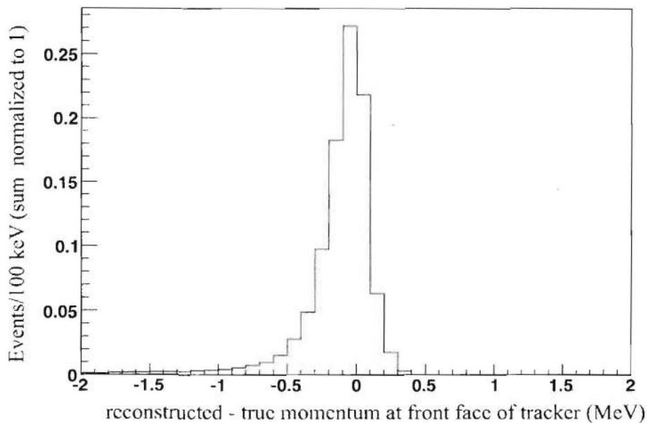
Figure 3.11: The distribution of (reconstructed - true) momentum for conversion events at the tracker, in MeV/c. The low-side tail demonstrates that DIO events with momenta near the conversion momentum are smeared away from the signal region. The sum of all events is normalized to unity.
