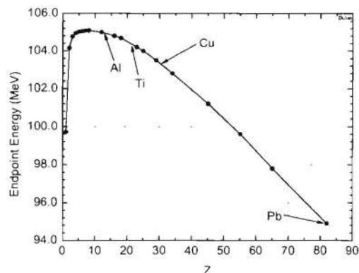
Figure 10.3: The muon decay-in-orbit endpoint energy vs Z.
