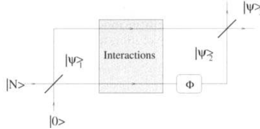
Figure 4. The second scheme for creating Schrödinger cat states with Bose condensates.
