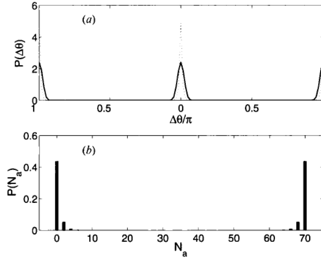
Figure 7. (a) Relative phase distribution for the optimally number squeezed state with N = 100 (dotted curve) and the phase distribution after the loss of 30 atoms (solid curve). (b) The final number distribution of mode a after phase shifting and Raman coupling. Despite significant loss, this is still a good approximation to a cat state.
