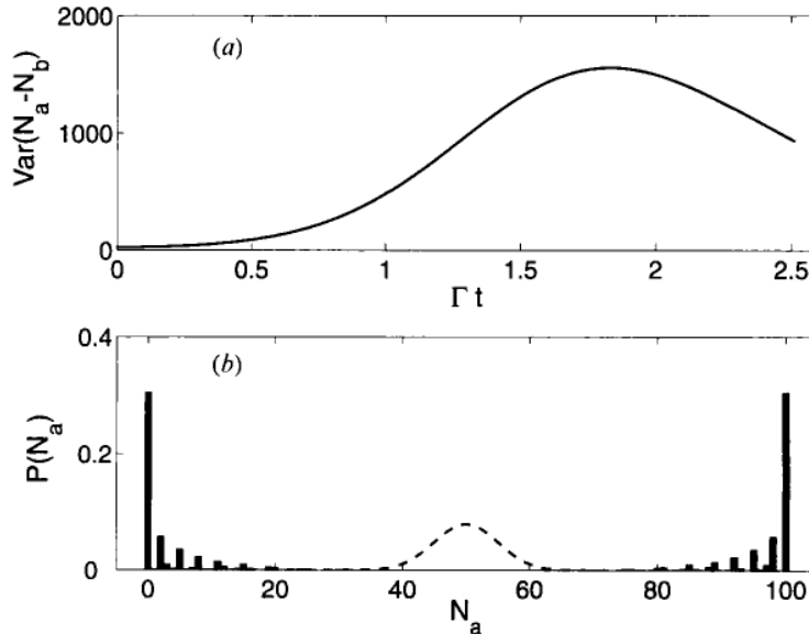
Figure 1. (a) Variance of (N_a - N_b) as a function of \Gamma t . (b) Number distribution of mode a at the optimum cat time (bar graph) compared with the initial number distribution (broken curve).
