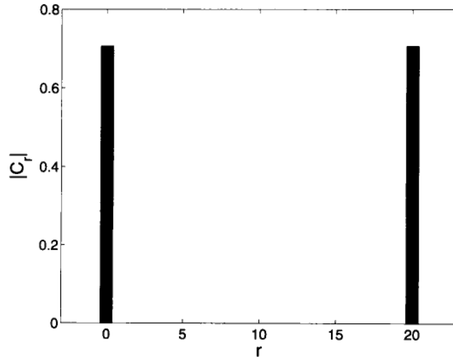
Figure 6. Plot of the modulus of the coefficients, C_r , of the final state, |\psi\rangle_3 for N = 20 . We see that the only non-vanishing coefficients are C_0 and C_{20} .
