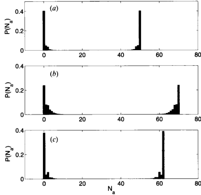
Figure 8. The final number distributions for mode a after the cat state generation scheme for (a) loss of 50 atoms after squeezing; (b) squeezing the initial state for only 1/\sqrt{2} of the optimum time and then loss of 30 atoms; (c) loss of 8% of the atoms during the squeezing time, then loss of a further 30 atoms afterwards.
