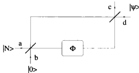
Figure 3. The interferometry scheme. An input state |N\rangle is coupled to a vacuum, |0\rangle , one arm is subjected to a phase shift, \phi , and then the two components are recombined. The output state is |\psi\rangle .
