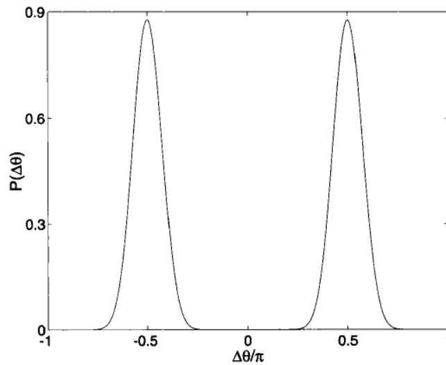
Figure 5. Plot of the phase distribution of |\psi\rangle_2 for N = 20 .
