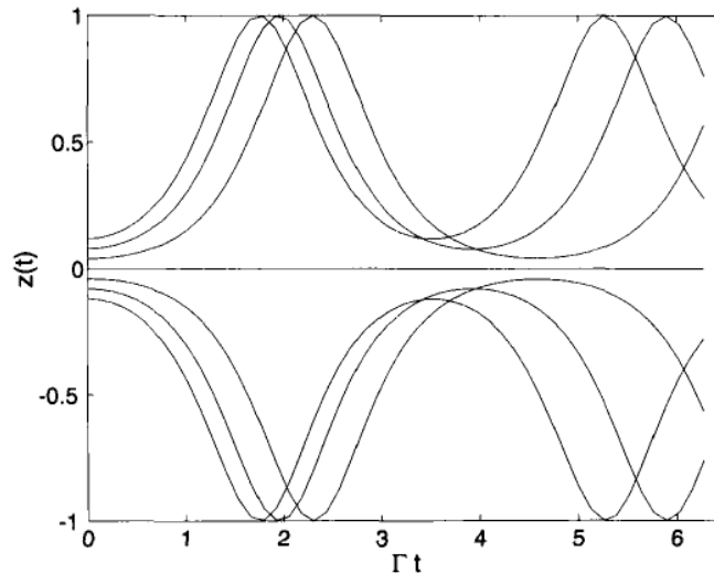
Figure 2. Solutions for z(t) of the semiclassical equations for the initial conditions \phi = 0 and z(0) \in \{-0.12, -0.08, -0.04, 0, 0.04, 0.08, 0.12\} .
