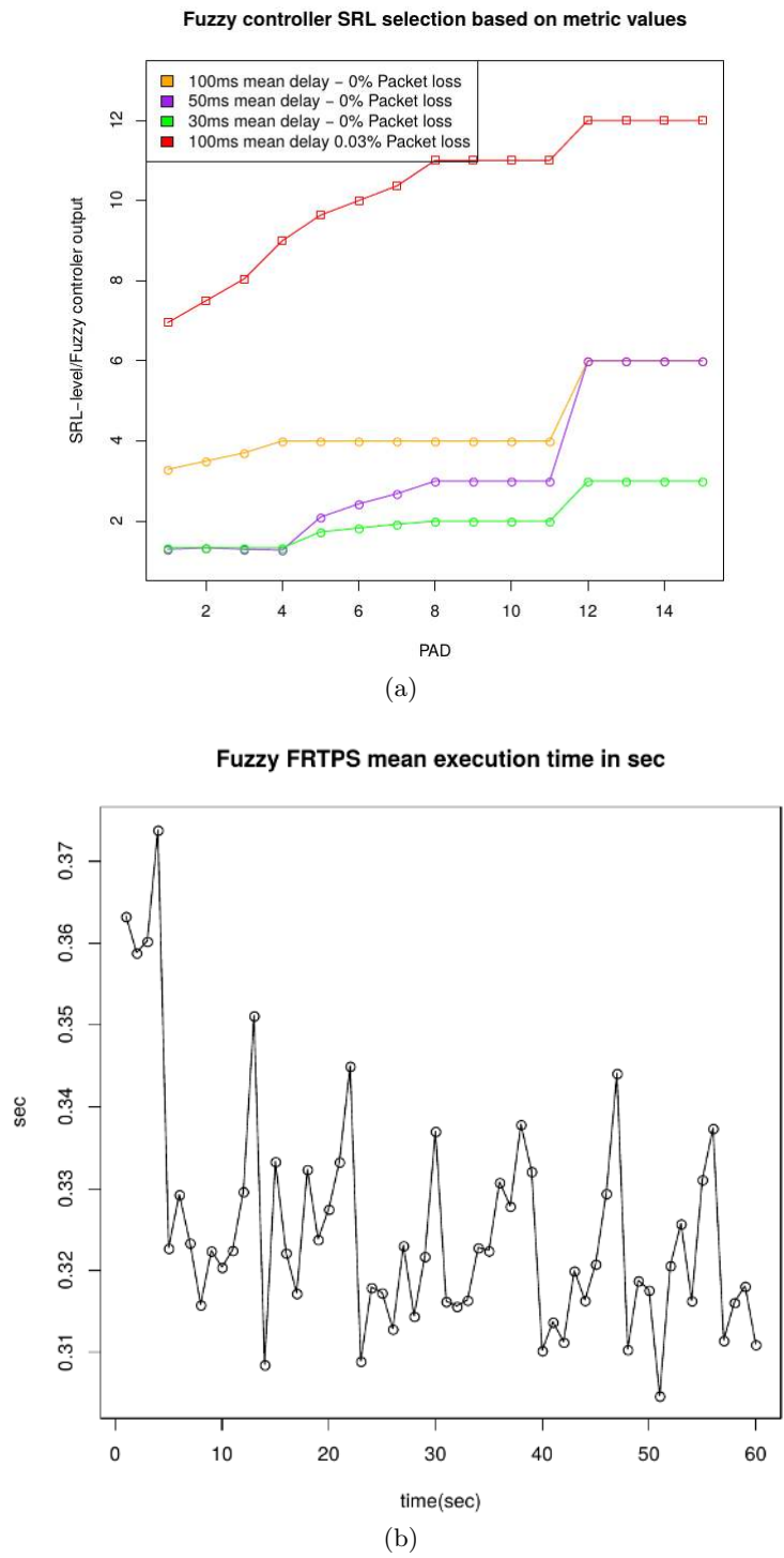
Figure 6: (a) FRTPS fuzzy states traversal over different estimated PAD values by the client - x axis in (ms) (b) FRTPS controller mean processing delay
