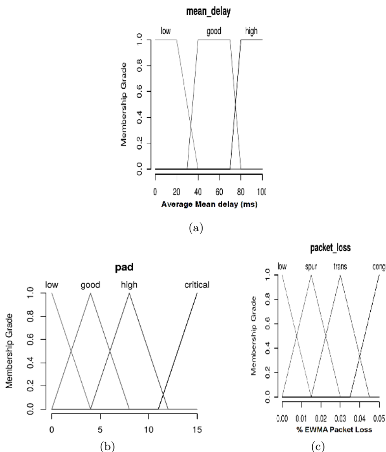
Figure 3: (a) FRTPS MF Fuzzy states for average Mean Delay (MD) - x axis in (ms) (b) FRTPS MS Fuzzy states for Packet Arrival Deviation (PAD) - x axis in (ms) (c) FRTPS MF Fuzzy states for Packet Loss (PLOSS) - x axis, % frame loss after EWMA process
