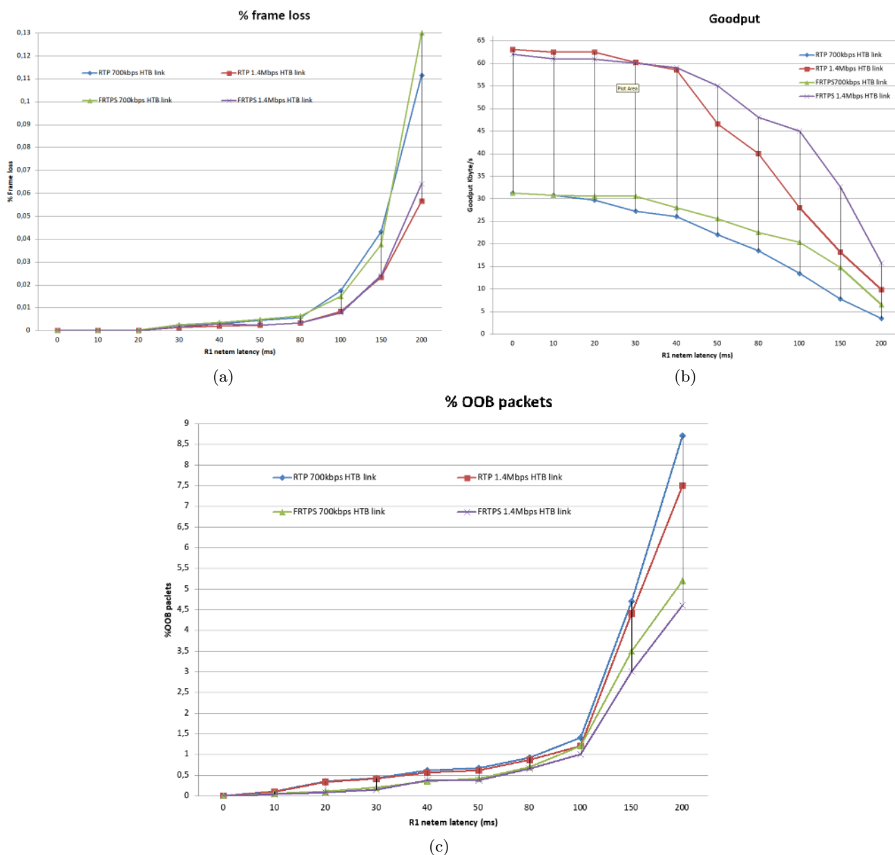
Figure 7: (a) %Frame Loss vs R1 Latency for 700kbps, 1,4Mbps channel capacity for the RTP and the FRTPS protocols. (b) Goodput Kbytes/s vs R1 Latency for 700kbps, 1,4Mbps channel capacity for the RTP and the FRTPS protocols. (c) % Packets out of Order vs R1 Latency for 700kbps, 1,4Mbps channel capacity for the RTP and the FRTPS protocols.
