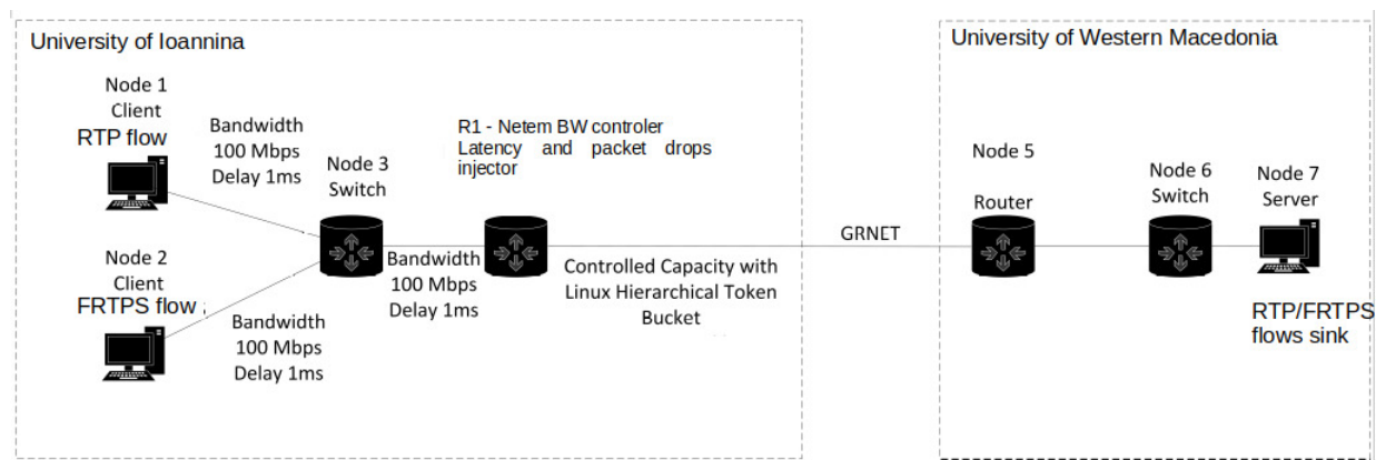
Figure 5: Network Topology of the performance evaluation scenario
