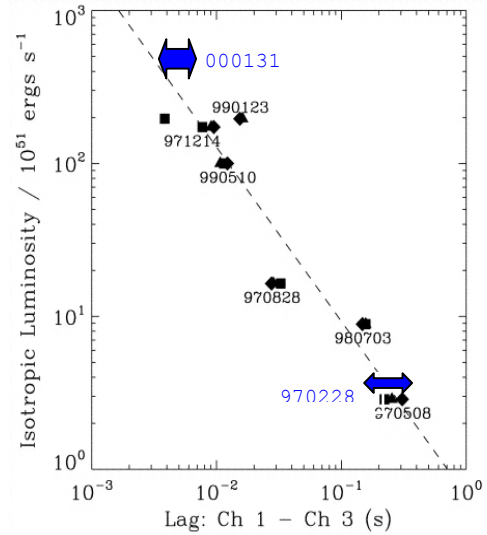
FIGURE 4. Luminosity-lag relation for GRBs (adapted from [7]). The observed correlation, L_{pk} \propto \Delta\tau^{-1.14} , may be understood as a kinematic effect from beaming [8].
