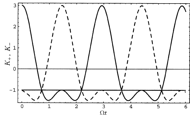
FIG. 1. Functions K_+ and K_- (dashed) versus \Omega t for the ideal case T=0 . Violations of Leggett-Garg-type inequalities occur whenever either curve goes below -1 .
