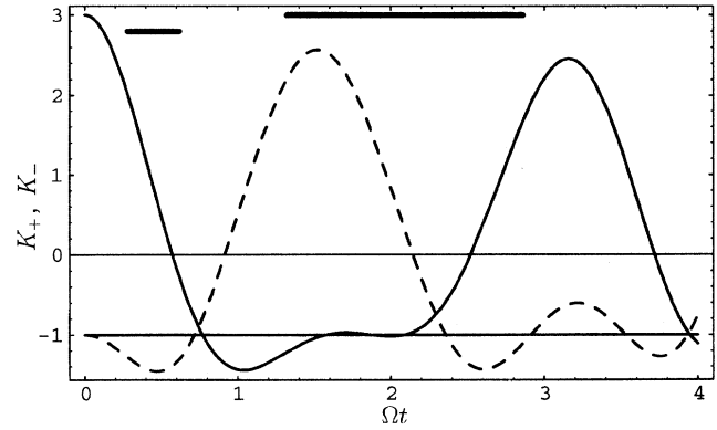
FIG. 3. K_{\pm} versus \Omega t at T=0.5 K. Violations of Leggett-Garg-type inequalities occur whenever either curve goes below -1 . The thick horizontal segments indicate the ranges of interaction times currently accessible for the two Rydberg transitions.
