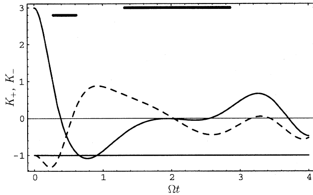
FIG. 2. K_{\pm} versus \Omega t at T=3 K. Violations of Leggett-Garg-type inequalities occur whenever either curve goes below -1 . The thick horizontal segments indicate the ranges of interaction times currently accessible for the two Rydberg transitions.
