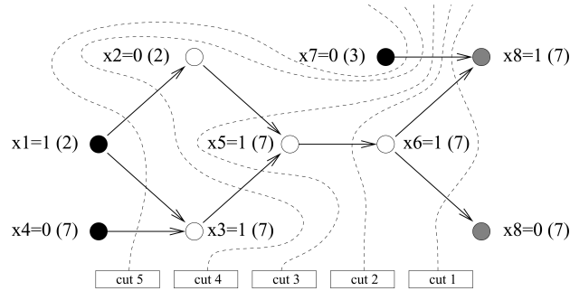
Fig. 10. Conflict-based learning based on the implication graph. Candidate learned clauses correspond to cuts between the decision assignments (black) and the conflicting assignments (right-hand side).
