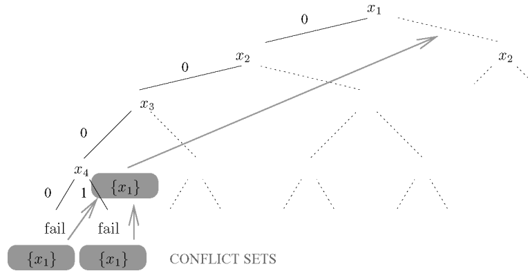
Fig. 14. Effect of maintaining conflict sets during the search. We detect the true reasons of the inconsistency of the branch on the left-hand side, and we can directly backjump to the branching level of variable x_1 . The conflict was caused by the choice x_1 = 0 , and is independent on whether value 0 or 1 is assigned to x_2 and x_3 .
