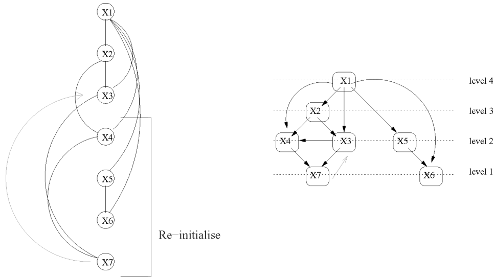
Fig. 16. Conflict directed backjumping. Sequential versus distributed settings.
