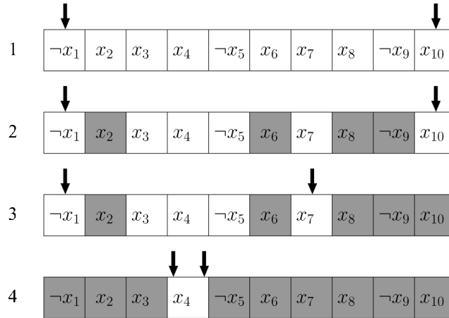
Fig. 4. Head/tails approach to BCP. For simplicity, we consider a clause on the variables x_1 \dots x_{10} . Darkened cells correspond to value 0 literals, while empty ones are free. (1) Initially head and tail pointers point to the beginning and the end of the array, respectively. (2) No action is needed in reaction to new assignments as long as they do not affect the head and tail literals (here the events x_2 = 0, x_6 = 0, x_8 = 0, x_9 = 1 have occurred). (3) If the literal pointed to by the tail pointer becomes 0, the pointer is moved left until it finds a free or value 1 cell (here we react to the event x_{10} = 0 ); the head pointer would similarly move right. (4) When the two pointers are at the same position, we have a unit clause if the cell is free, and we have a conflict if it has value 0 (here the events x_1 = 1, x_3 = 0 and x_7 = 0 have occurred, we have a unit clause).
