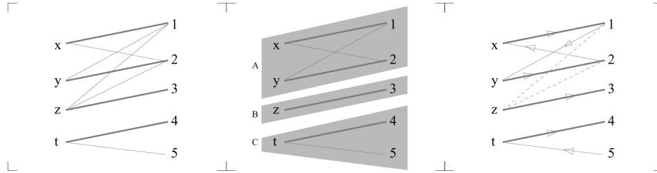
Fig. 8. Régin's propagation algorithm [1974] for the alldiff constraint.
