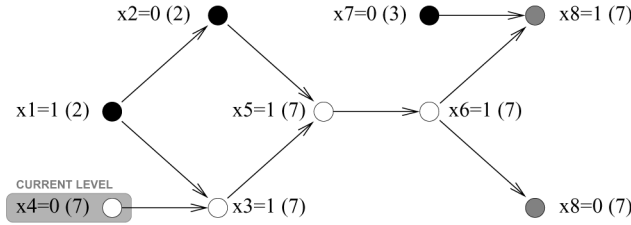
Fig. 9. Implication graph. The numbers in parenthesis are the decision levels of each assignment. The nodes in black correspond to assignments done at previous levels. The conflicting assignments are those on the right-hand side.
