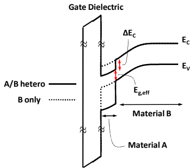
Fig. 20. The effective tunneling band gap in Type II heterojunction is smaller than those of A and B alone [9].
