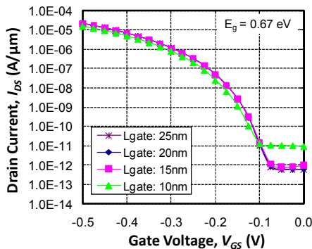
Fig. 23. Simulated gFET IV is insensitive to L_G variation because the tunneling region is in the N+ source, protected from the drain.
