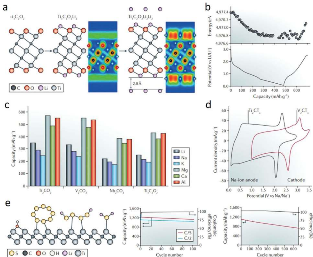
Fig. 8 MXenes as conductive electrodes in batteries. a Schematic representation of Li^+ insertion in the Ti_3C_2T_x . Without and with the extra lithium film, the valence electron localization functions are described. b Edge energy variation of titanium versus capacity of MXene during delithiation and lithiation process integrated along the analogous voltage contours. c On the oxygen-terminated MXene sheets, theoretical capacities of nonlithium and lithium ions were theoretically obtained. a–c reprinted with permission from 38 JACS 2014, 136, 17, 6385–6394; Publication Date: March 28, (2014) https://doi.org/10.1021/ja501520b Copyright (2014) American Chemical Society; (d) Cyclic voltammetry (CV) curves of V_2C and Ti_2C in a Na^+ electrolyte. d reprinted with permission from 106 The journal of physical chemistry letters 2015, 6, 2305–2309; Publication Date: June 5, (2015) https://doi.org/10.1021/acs.jpcllett.5b00868 Copyright (2015) American Chemical Society; e Performance representation of Ti_2C-S MXene composite in Li-S batteries; A graphical demonstration of the substitution of the Ti-OH bond with S-Ti-C bond on the MXene surface upon treatment by heat or contacting with polysulfides (presented on the leftward); the cyclic functioning of a 70 wt% d-Ti_2C-S MXene composite at C/2 and C/5 (in middle); and long-period cycling at C/2 is presented on the rightward. Reprinted with permission from 112 .
