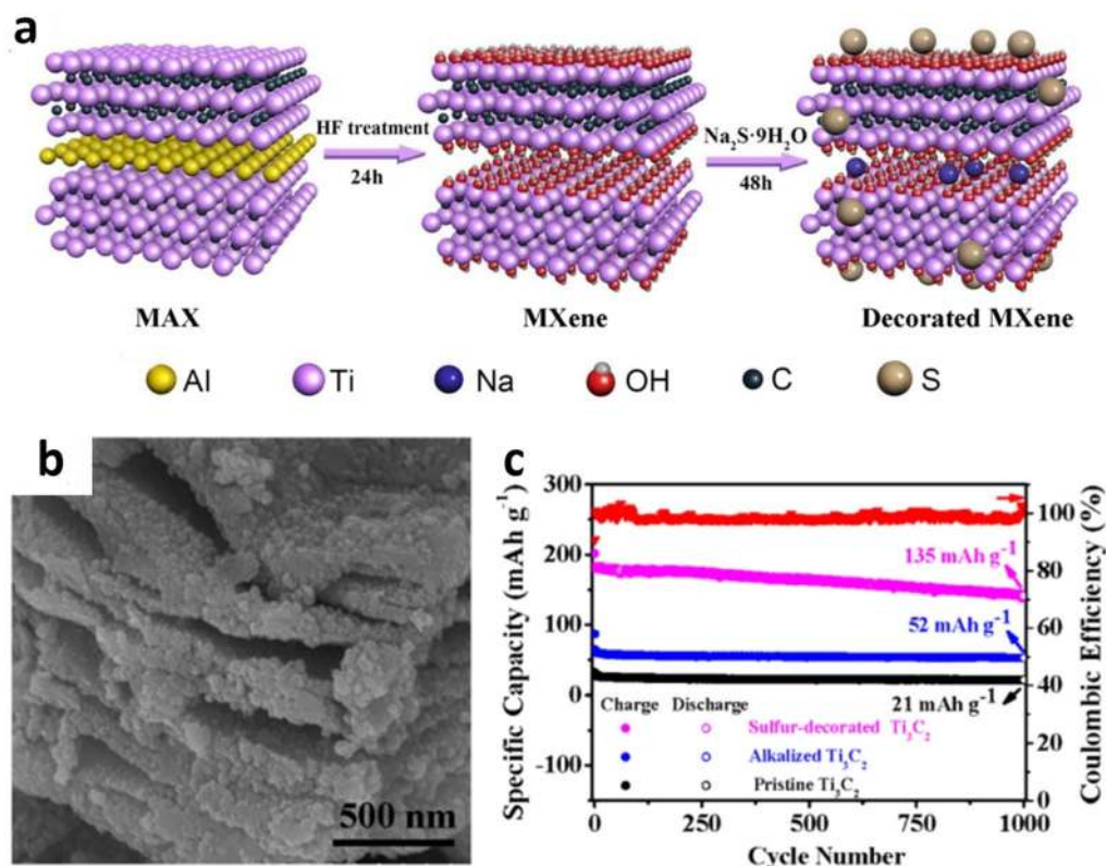
Fig. 11 Performance of sulfur-decorated Ti_3C_2 MXene. a Graphical representation of the synthesis of S-decorated Ti_3C_2 MXenes. b SEM image of S- Ti_3C_2 MXenes. c Cycling performance and coulombic efficiencies S- Ti_3C_2 MXenes and alkali-rich Ti_3C_2 MXenes at a current density of 2 A g^{-1} . a–c used with permission from Elsevier B.V./Sun 150 .
