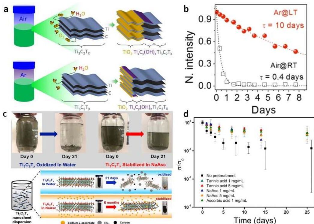
Fig. 13 Shelf stability of colloidal MXenes. a Schematic diagram of colloidal d\text{-Ti}_3\text{C}_2\text{T}_x MXene aqueous solution degradation in the air and argon at room temperature denoted as Air@RT and Ar@RT. b The d\text{-Ti}_3\text{C}_2\text{T}_x stability in Air@RT and Ar@LT. a, b reprinted with permission from 157 Chemistry of Materials 2017, 29, 4848-4856; Publication Date: May 09, (2017) https://doi.org/10.1021/acs.chemmater.7b00745 Copyright (2017) American Chemical Society; c Shelf-stable \text{Ti}_3\text{C}_2\text{T}_x NSs stabilized by sodium L-ascorbate (NaAsc) solution and stored in deionized water. \text{Ti}_3\text{C}_2\text{T}_x oxidizes and degrades without antioxidants to form \text{TiO}_2 and carbon. Sodium L-ascorbate protects against seriously oxidizing the nanosheet; d Conductivity shift vs. time of \text{Ti}_3\text{C}_2\text{T}_x Buckypaper produced after pretreatment with selected antioxidants. c, d used with permission from Elsevier B.V./Zhao 158 .
