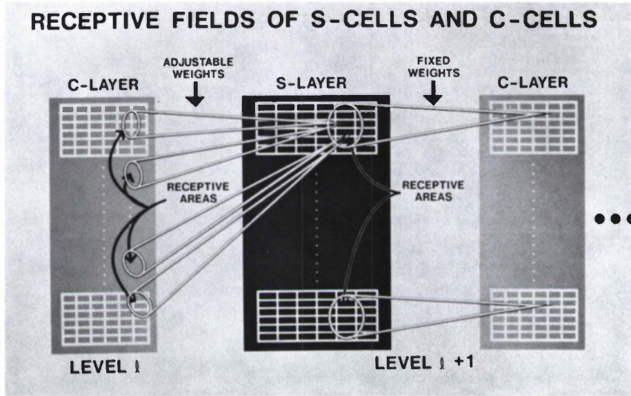
Figure 2-3. Interconnection architecture of the Neocognitron.
