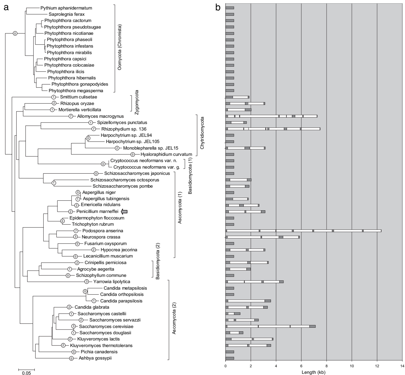
Fig. 1. Number, size, and position of introns in CO1 of fungi and fungus-like Oomycota. (a) Neighbor-joining tree of 56 fungal species for which complete mitochondrial genomes and/or complete CO1 genes are available in GenBank. The tree is constructed with the 648-bp CO1 barcode region. The circled numbers indicate the number of introns in the barcode region for all taxa to the right of the symbol, and the arrow indicates the approximate taxonomic location of the fine-scale analysis. (b) Exon and intron lengths in the 648-bp CO1 barcode region for the 56 fungal species. Exons are shaded dark gray, and introns are shaded white. Exon-intron boundaries are based on annotations provided by the GenBank records.
