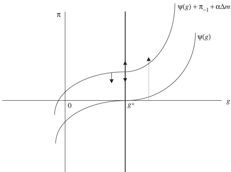
Figure 3: Inflation Model
