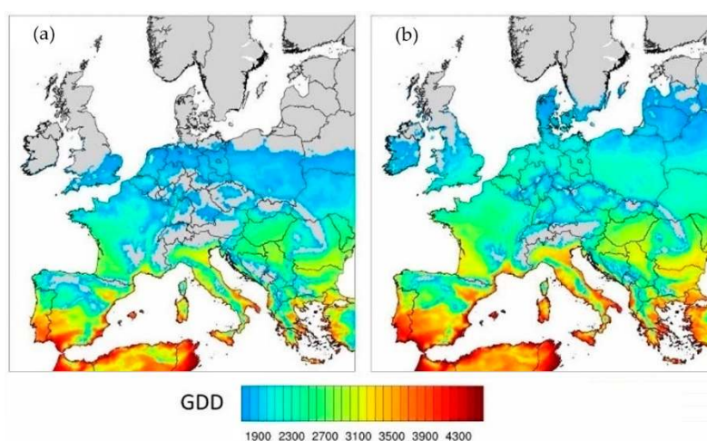
Figure 5. Current (years 1970–2000) (a) and projected (years 2070–2100) (b) thermal time (in growth degree days, GDD) under the RCP8.5 scenario in Europe. The base temperature is set at 10 °C which applies to the requirements of C4-crops such as miscanthus ( Miscanthus × giganteus Greef et Deuter) and maize ( Zea mays L.).
