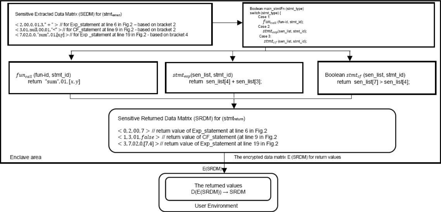
Figure 3 The partitioned statements of the Java program in Fig. 2 and their execution process inside the enclave
