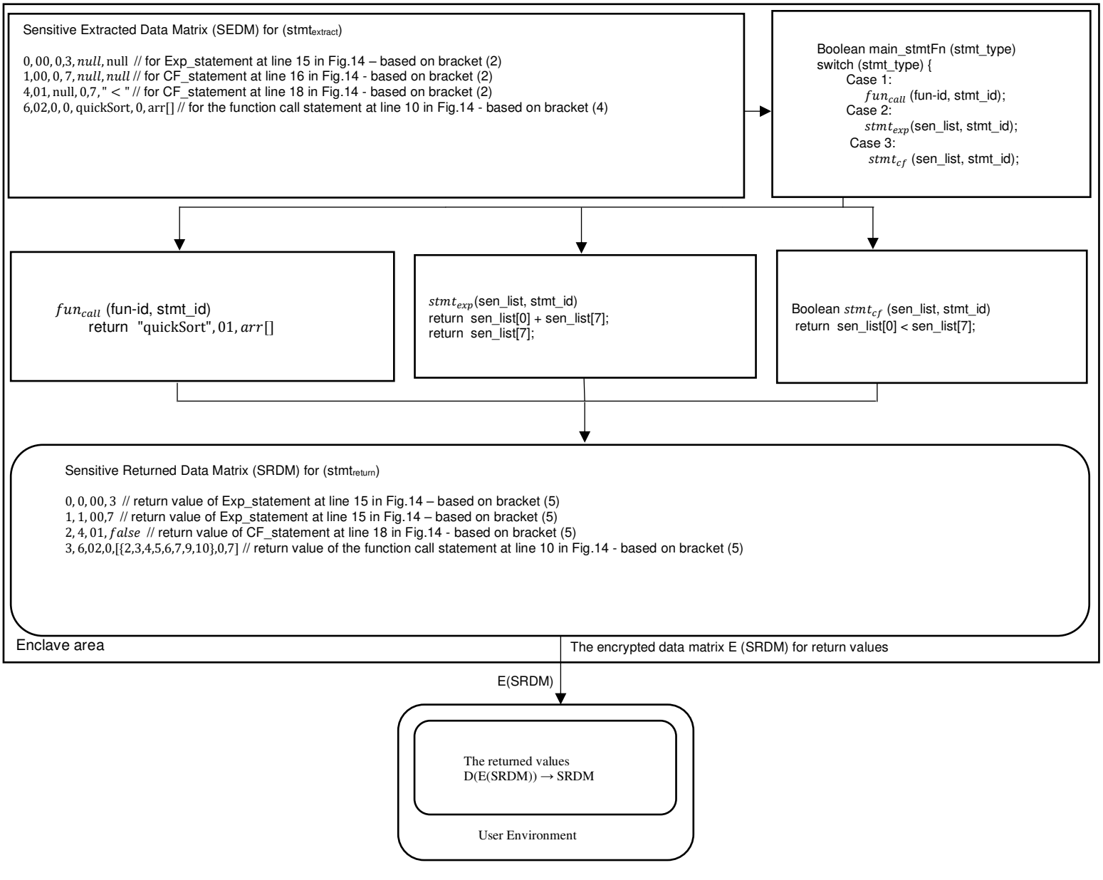
Fig .16 Execution process of QuickSort application inside/outside the enclave
