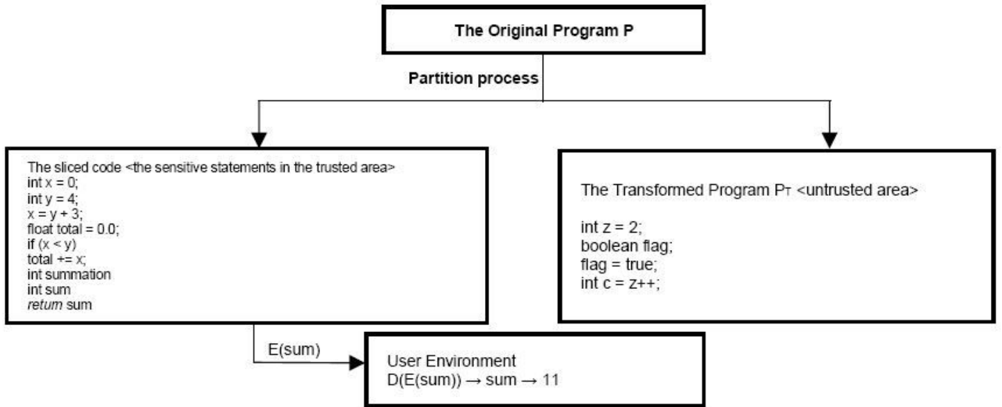
Figure 3 The partitioned statements of the Java program in Fig. 2 and their execution process inside the enclave
