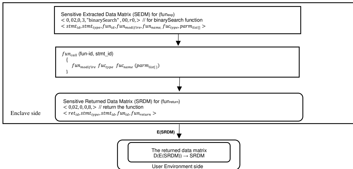
Fig. 8 The process execution sequence of the binary search functions inside and outside the enclave.
