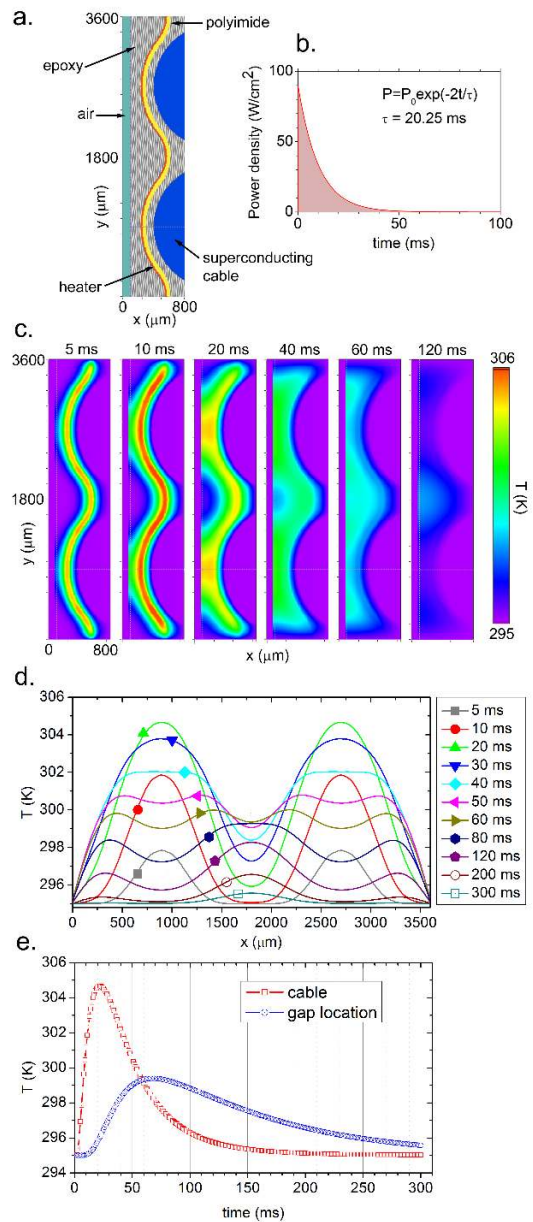
Fig. 2. (a) Heater stack setup used for the 2D heat diffusion simulation. (b) Time dependence of the heater power assumed for the simulation (c) A sequence of 2D heat maps calculated at various time intervals from the onset of heater firing. (d) Temperature profiles calculated along the outer surface of the heater stack at various time intervals. Surface temperature peaks initially seen at the locations where heater layer is pushed towards the stack surface, gradually transform into “dips” as heat is being removed into the underlying cable turns. (e) Time dependences of surface temperature at y=900 \mu m (cable location) and y=1800 \mu m (gap between the cable turns). Temperature peaks sequentially in those locations with a \sim 50 ms interval. Characteristic thermal relaxation times constants past the peak are \sim 35 ms and \sim 127 ms respectively.
