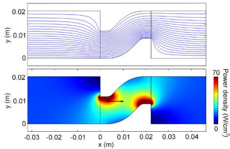
Fig. 3. (a) Result of a simulation for the current flow lines (top) and surface power distribution (bottom) in a single period of a heater strip of variable cross-section. Power deposition peaks locally at the curvature end points. A relative temperature rise from the middle of the heating station towards the hot spot along the central line (depicted with an arrow) is \sim 58\%
