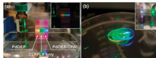
Fig. 24 Polyurethane polymer samples containing PdOEP and DPA irradiated by 532 nm green laser. Modified and reprinted with permission from ref. 83. Copyright 2012 American Chemical Society. http://pubs.acs.org/doi/full/10.1021/cm3012414 .
