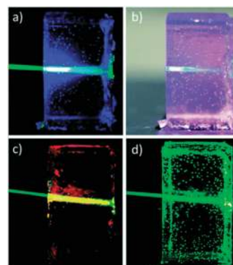
Fig. 23 Organogels based on PVOH–HMDI/DMF/DMSO under irradiation with 543 nm laser. (a and b) Gels containing PdMesolIX ( 2 \times 10^{-5} M) and DPA ( 10^{-2} M). (c and d) Gels containing only PdMesolIX ( 2 \times 10^{-5} M) or DPA ( 10^{-2} M) respectively. Reproduced from ref. 74 with permission from the Royal Society of Chemistry.
