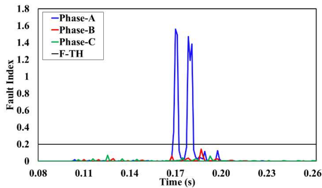
FIGURE 14. AG fault detection for Arcing phenomenon.
