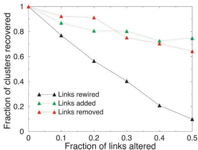
Fig. 5. The fraction of clusters recovered in the randomly perturbed network, as a function of the fraction of altered links. Black curves correspond to the case when links are randomly rewired; red, randomly removed (true negatives); and green, randomly added (false positives). The original cluster is said to be recovered if the perturbed network has a cluster that shares at least 50% of the nodes with the original one. Each perturbation was repeated 10 times. Also see Fig. 9, which is published as supporting information on the PNAS web site.
