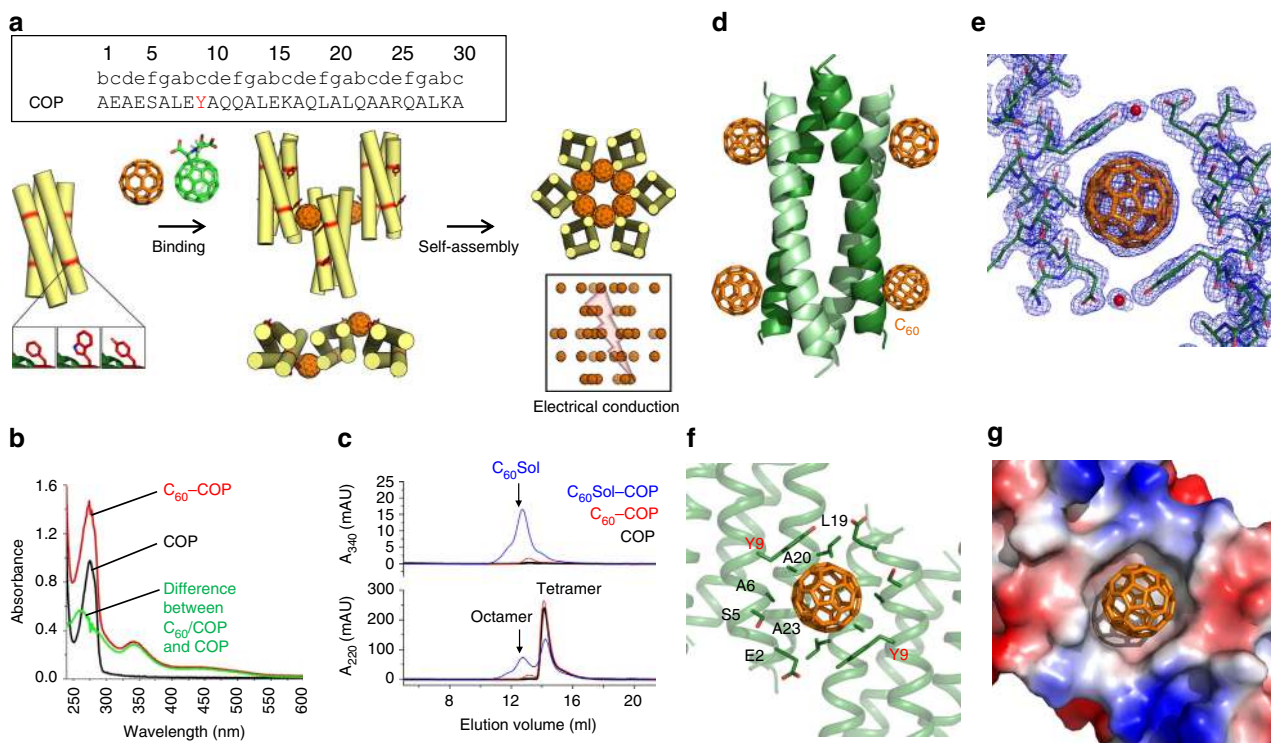
Figure 1 | Protein/C 60 super-assembly. (a) COP, a stable tetramer in isolation, interacts with C 60 moieties by means of a surface-binding site that includes Tyr residues (other aromatic side chains also likely admissible), and further self-assembles into a co-crystalline array with fullerene. (b) Ultraviolet absorption spectra of a C 60 /COP suspension and COP alone demonstrate that primitive fullerene (green) dissolves in the aqueous phase in the presence of protein. (c) SEC traces of COP alone or in association with C 60 or C 60 Sol. Top and bottom plots show absorbances at 340 and 220 nm, respectively. The lower-retention peaks arising due to the addition of C 60 or C 60 Sol are consistent with the molecular weight of a COP octamer (for example, dimer of tetramers; Supplementary Fig. 10). (d) Each COP tetramer in the C 60 Sol-COP crystal is associated with four fullerenes (one per chain), each fullerene being wedged between two adjacent COP tetramers, for an overall stoichiometry of two fullerenes for one COP tetramers. (e) Omit map (2F o - F c , contoured at 1.2σ) showing electron density of the C 60 group (orange sticks) sandwiched via π-π stacking between Tyr residues from adjacent COPs. (f) Residues involved in C 60 coordination are shown with sticks and labelled. (g) Surface representation of the C 60 coordination site, coloured in vacuo electrostatic potential (red to blue corresponds to negative-to-positive relative potentials).
