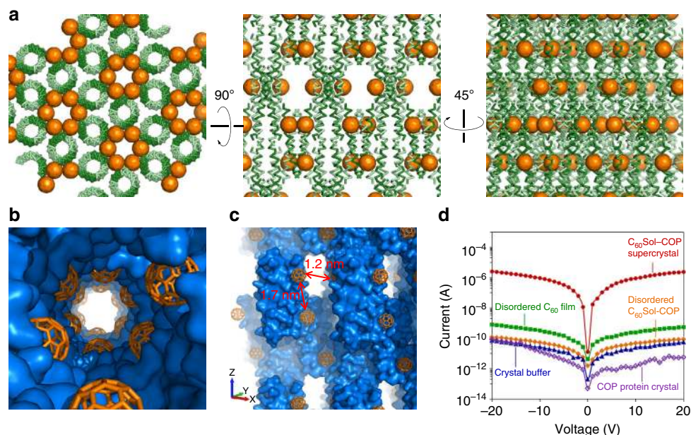
Figure 3 | Assembly of fullerenes endsows crystal with electronic transport capabilities. (a) Three views of the C_{60} Sol-COP crystal lattice. (b) C_{60} groups are arranged in a helical manner along parallel inner channels in the assembly. (c) A side view of the channel showing nearest-neighbor inter- C_{60} distances. (d) Semi-logarithmic current-voltage characteristic of C_{60} Sol-COP supercrystal (red dots) and disordered C_{60} Sol-COP (orange diamonds). Disordered C_{60} film dried from a bare C_{60} /toluene solution (green squares), crystal buffer solution (blue triangles) and a COP-alone protein crystal (violet open circles) were also characterized as controls.
